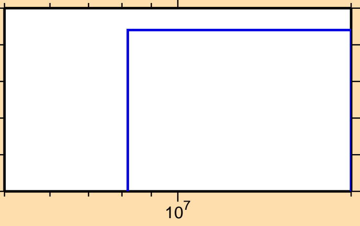
\sigma vs. E for ^{192}\text{Pb}(n,\text{He}3)
