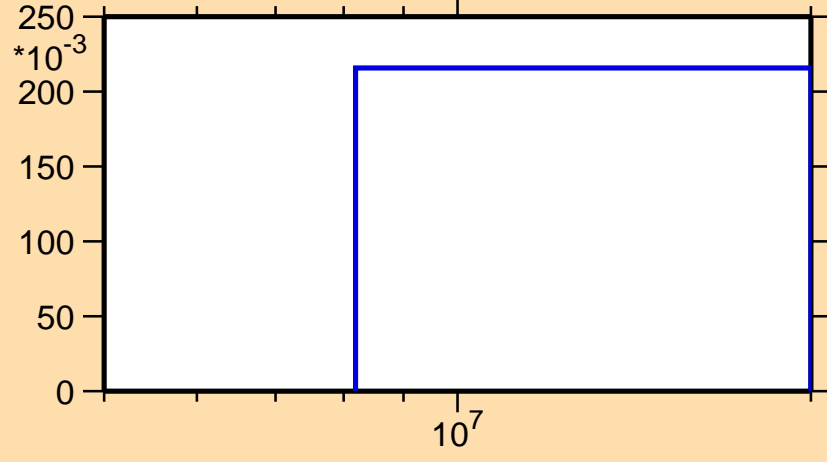
\sigma vs. E for ^{192}\text{Pb}(n,2n)
