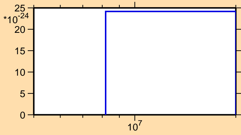
\sigma vs. E for ^{192}\text{Pb}(\text{mt } 11)
