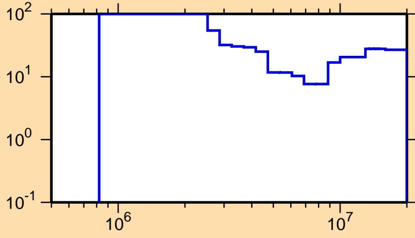
\Delta\sigma/\sigma vs. E for ^{193}\text{Pb}(n,n\text{cont.})
