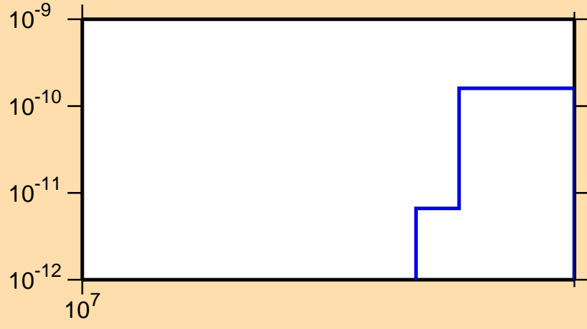
\sigma vs. E for ^{193}\text{Pb} (mt 34)
