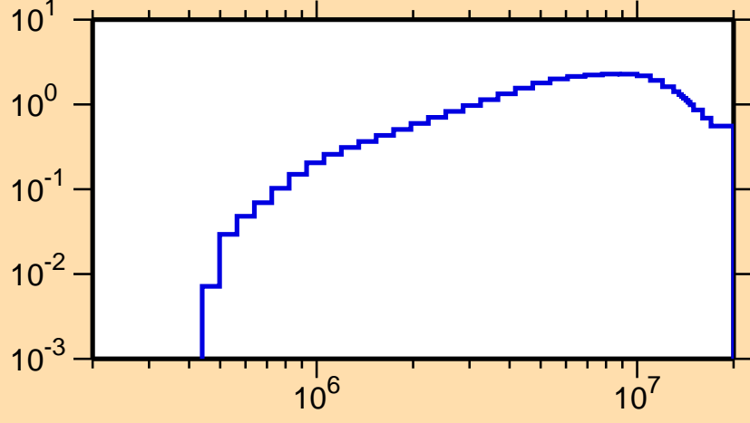
\sigma vs. E for ^{193}\text{Pb}(n,\text{inel.})
