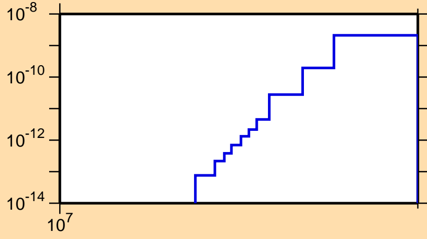
\sigma vs. E for ^{193}\text{Pb}(\text{mt } 45)
