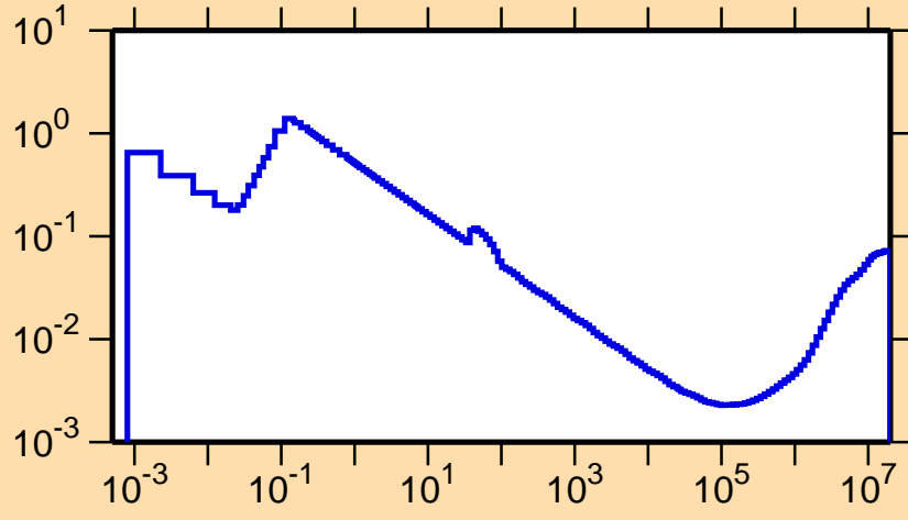
\sigma vs. E for ^{193}\text{Pb}(n,p)
