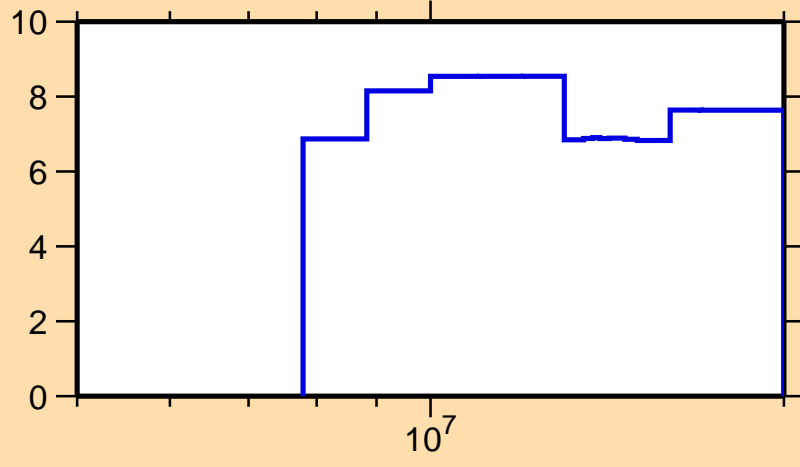
\Delta\sigma/\sigma vs. E for ^{193}\text{Pb}(n,\text{nonel.})
