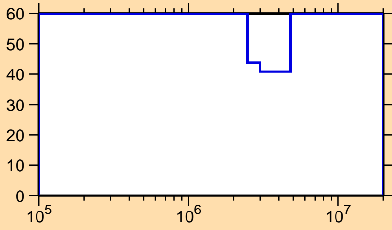
\Delta\sigma/\sigma vs. E for ^{193}\text{Pb}(n,n_1)
