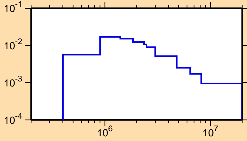
\sigma vs. E for ^{193}\text{Pb}(n,n_4)
