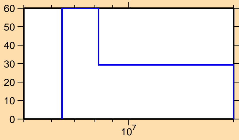
\Delta\sigma/\sigma vs. E for ^{193}\text{Pb}(n,2n)
