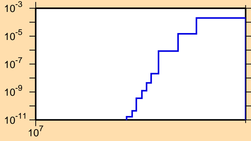
\sigma vs. E for ^{193}\text{Pb}(n,2np)
