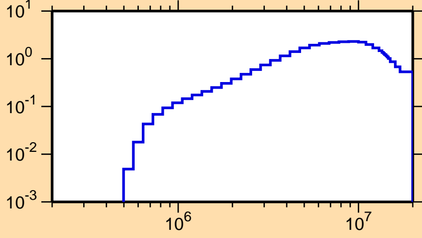
\sigma vs. E for ^{193}\text{Pb}(n,n\text{cont.})
