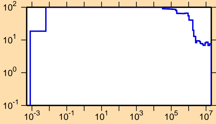
\Delta\sigma/\sigma vs. E for ^{193}\text{Pb}(n,\text{nonel.})
