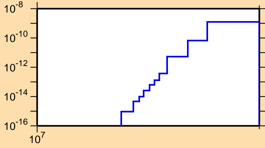
\sigma vs. E for ^{193}\text{Pb}(n,\text{pt})
