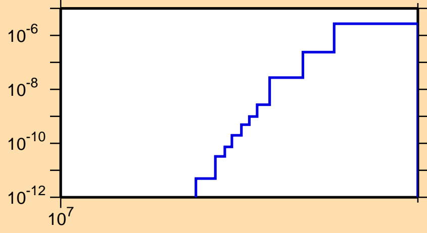
\sigma vs. E for ^{193}\text{Pb}(n,\text{nd})
