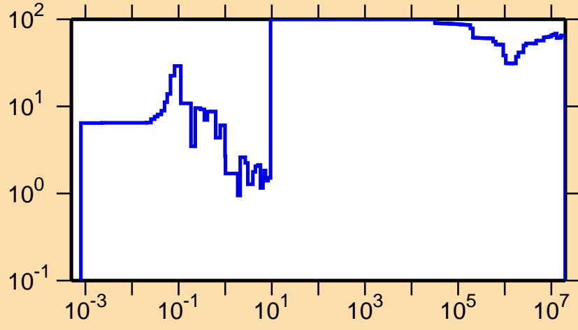
\Delta\sigma/\sigma vs. E for ^{193}\text{Pb}(n,\gamma)
