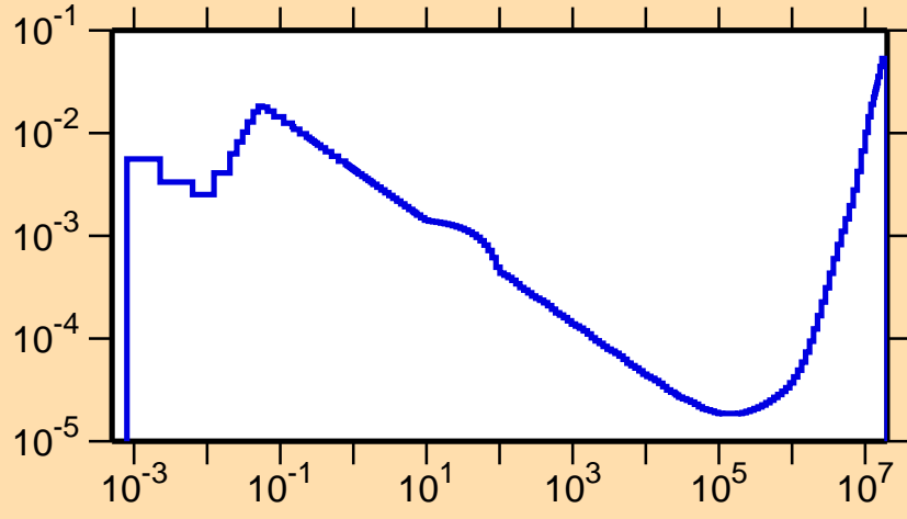
\sigma vs. E for ^{193}\text{Pb}(n,\alpha)
