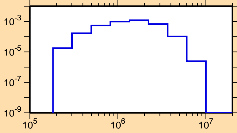
\sigma vs. E for ^{193}\text{Pb}(n,n_2)
