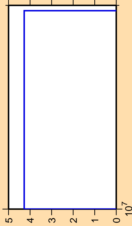
\Delta\sigma/\sigma vs. E for ^{193}\text{Pb}(\text{mt117})
