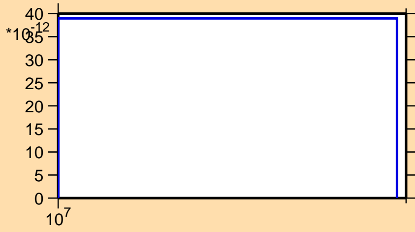
\sigma vs. E for ^{193}\text{Pb} (mt 45)
