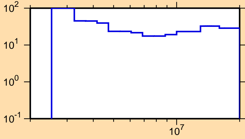
\Delta\sigma/\sigma vs. E for ^{194}\text{Pb}(n,n\text{cont.})
