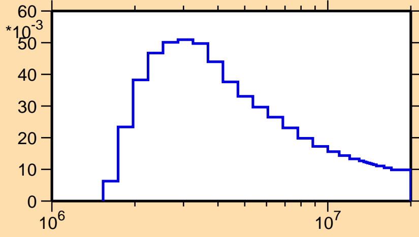
\sigma vs. E for ^{194}\text{Pb}(n,n_4)
