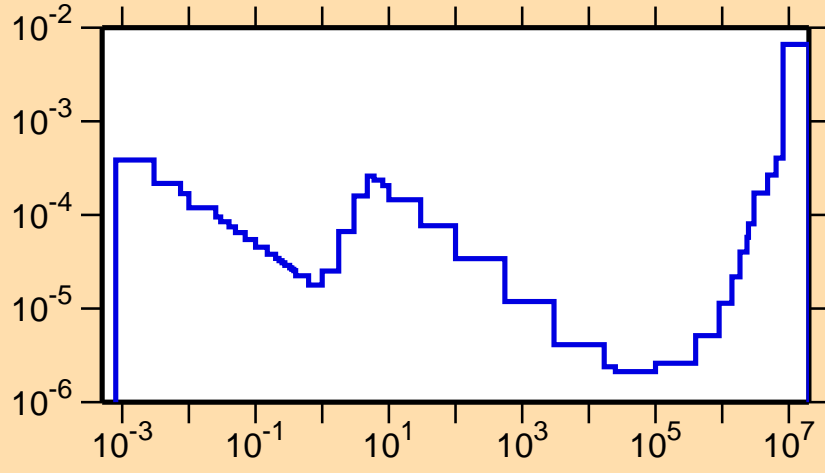
\sigma vs. E for ^{194}\text{Pb}(n,\alpha)
