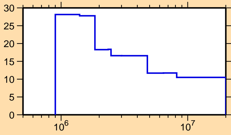
\Delta\sigma/\sigma vs. E for ^{194}\text{Pb}(n,\text{nonel.})
