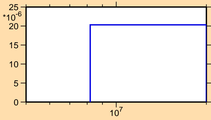
\sigma vs. E for ^{194}\text{Pb}(n,t)
