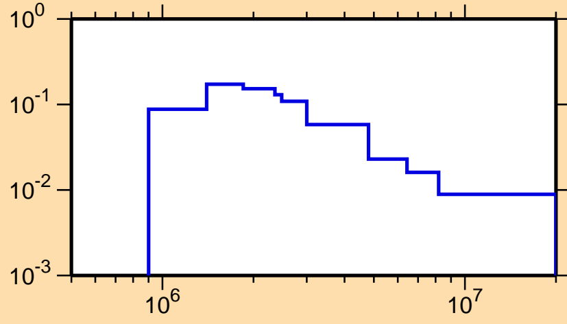
\sigma vs. E for ^{194}\text{Pb}(n,n_2)
