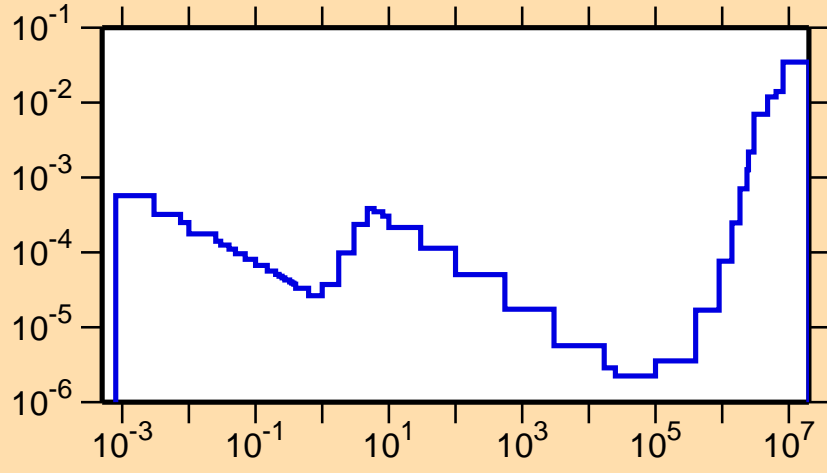
\sigma vs. E for ^{194}\text{Pb}(n,p)
