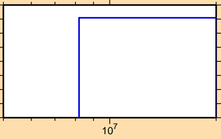
\sigma vs. E for ^{194}\text{Pb}(\text{mt } 45)
