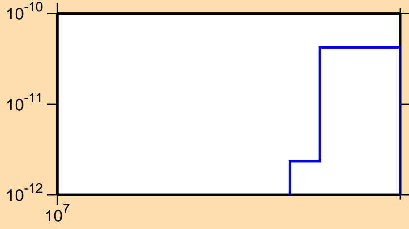
\sigma vs. E for ^{195}\text{Pb}(\text{mt } 45)
