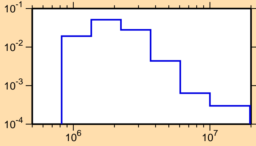
\sigma vs. E for ^{197}\text{Pb}(n,n_3)
