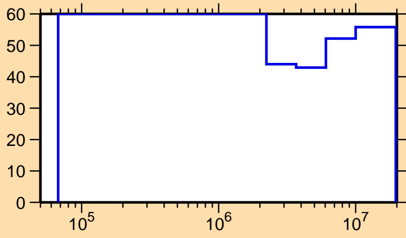
\Delta\sigma/\sigma vs. E for ^{197}\text{Pb}(n,n_1)
