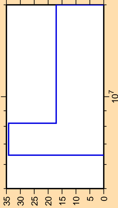
\Delta\sigma/\sigma vs. E for ^{197}\text{Pb}(n,\gamma)
