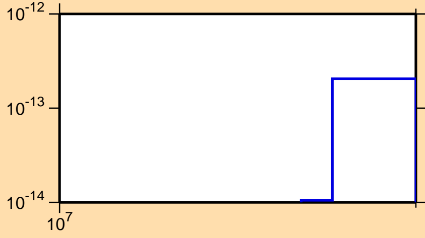
\sigma vs. E for ^{197}\text{Pb}(\text{mt117})
