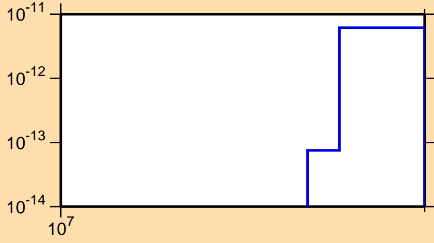
\sigma vs. E for ^{197}\text{Pb}(\text{mt } 34)
