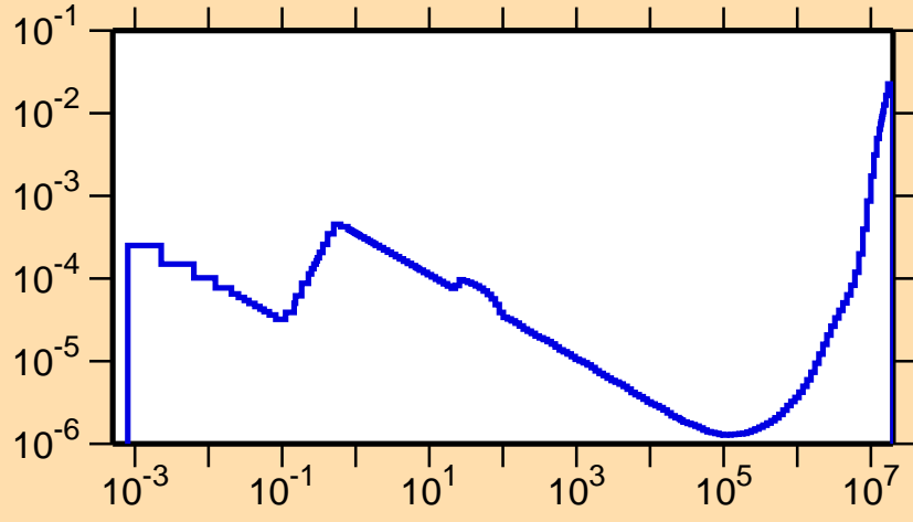
\sigma vs. E for ^{197}\text{Pb}(n,\alpha)
