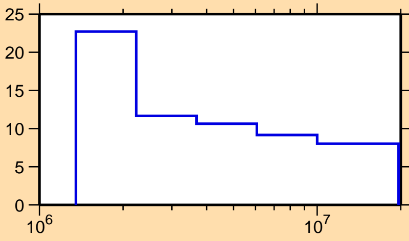
\Delta\sigma/\sigma vs. E for ^{197}\text{Pb}(n,n\text{onel.})
