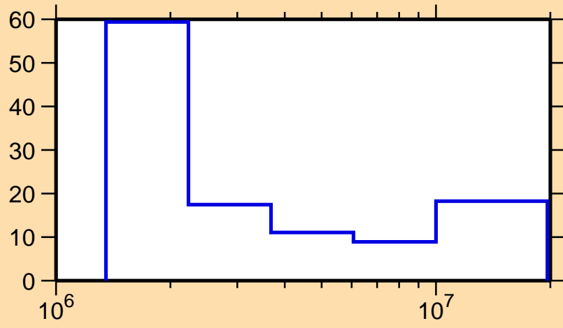
\Delta\sigma/\sigma vs. E for ^{197}\text{Pb}(n,n\text{cont.})
