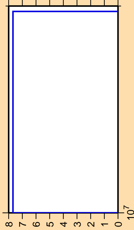
\Delta\sigma/\sigma vs. E for ^{197}\text{Pb}(n,\text{pd})
