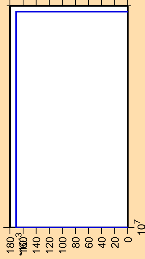
\Delta\sigma/\sigma vs. E for ^{197}\text{Pb}(\text{mt } 45)
