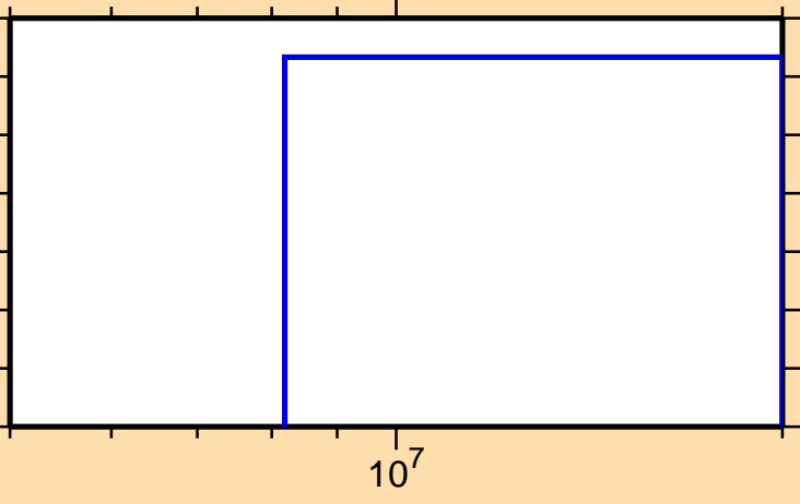
\sigma vs. E for ^{197}\text{Pb}(n,\text{pt})
