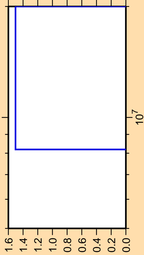
\Delta\sigma/\sigma vs. E for ^{198}\text{Pb}(n,pd)
