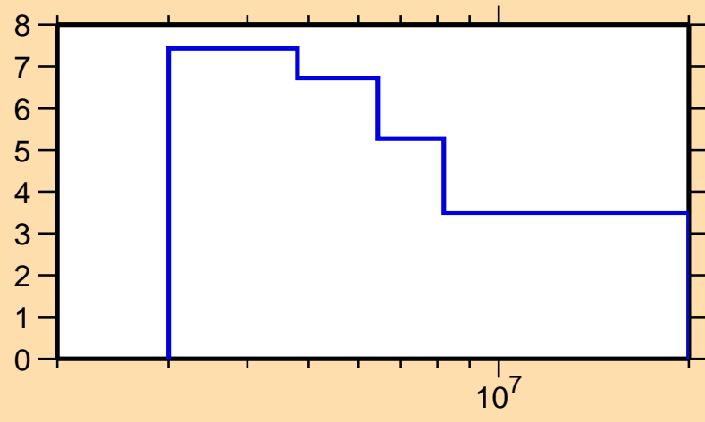
\Delta\sigma/\sigma vs. E for ^{198}\text{Pb}(n,\text{tot.})
