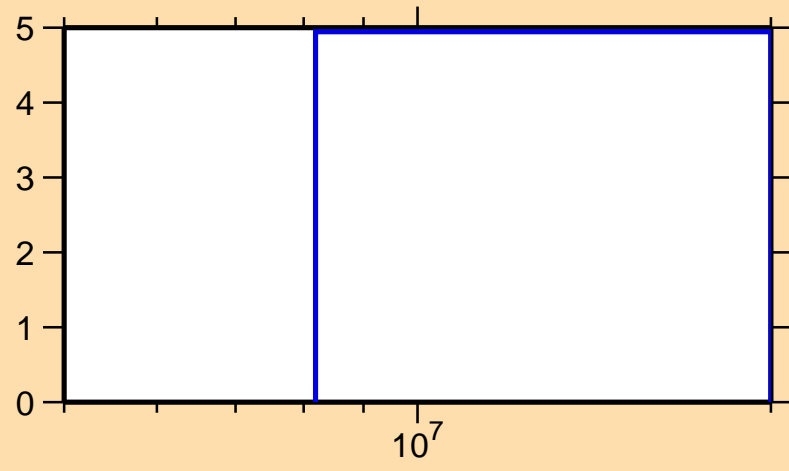
\Delta\sigma/\sigma vs. E for ^{198}\text{Pb}(n,\text{nonel.})
