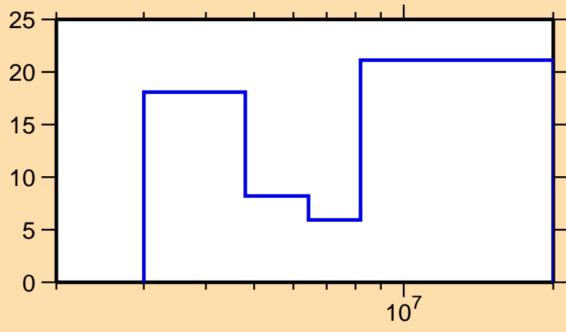
\Delta\sigma/\sigma vs. E for ^{198}\text{Pb}(n,\text{inel.})
