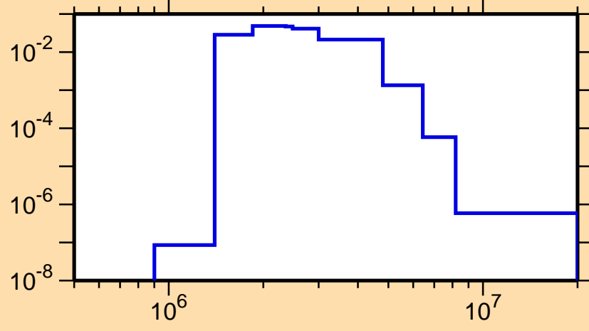
\sigma vs. E for ^{198}\text{Pb}(n,n_2)
