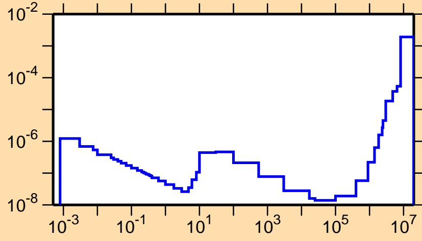
\sigma vs. E for ^{198}\text{Pb}(n,\alpha)
