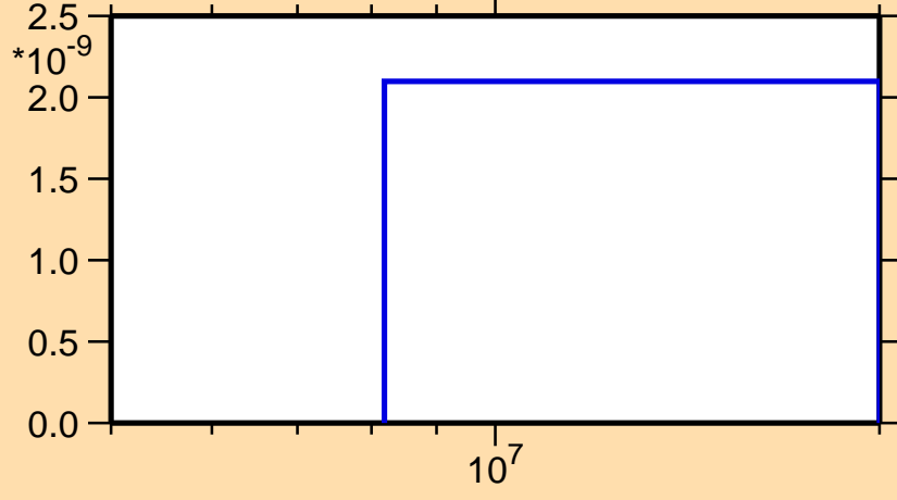
\sigma vs. E for ^{198}\text{Pb}(n,2np)
