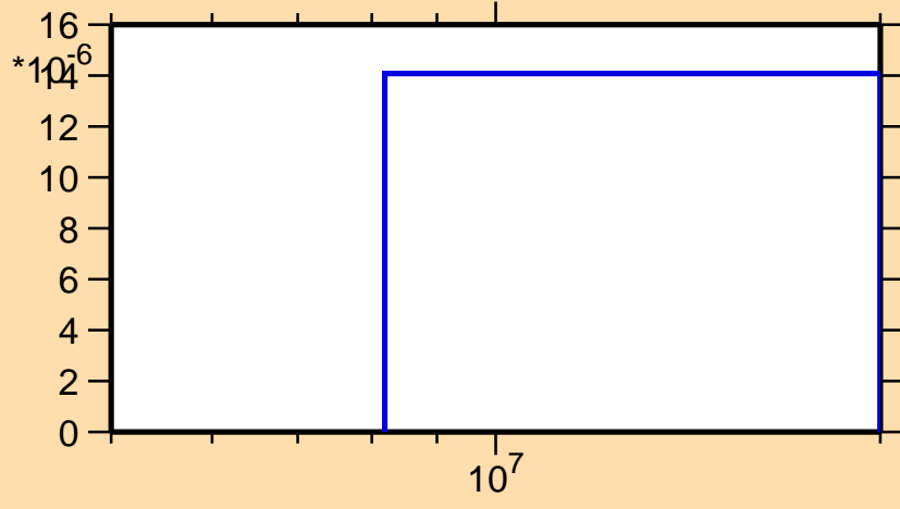
\sigma vs. E for ^{198}\text{Pb}(n,t)
