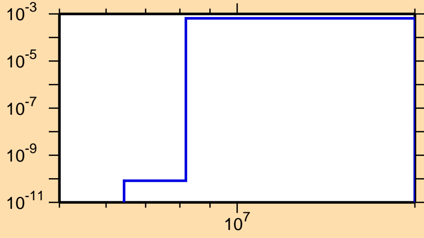
\sigma vs. E for ^{198}\text{Pb}(n,d)
