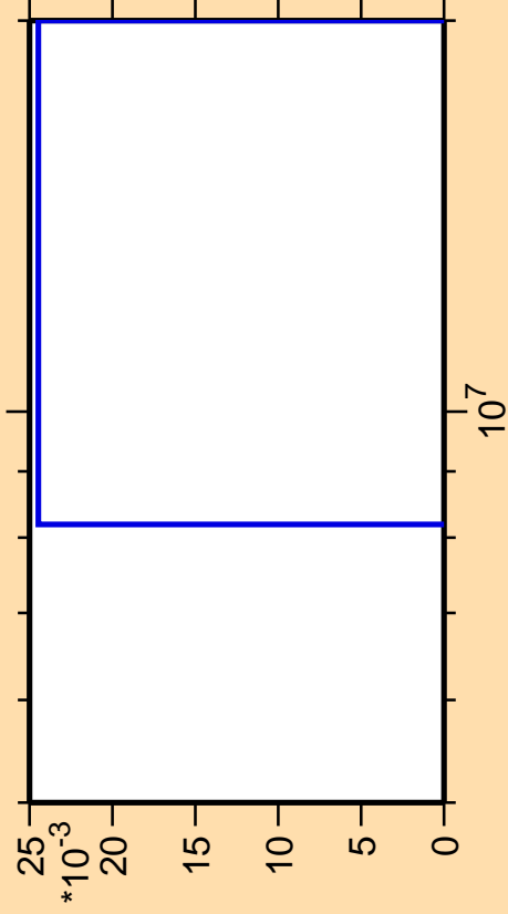
\Delta\sigma/\sigma vs. E for ^{198}\text{Pb}(\text{mt } 45)
