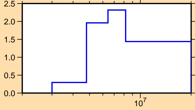
\sigma vs. E for ^{198}\text{Pb}(n,n\text{cont.})
