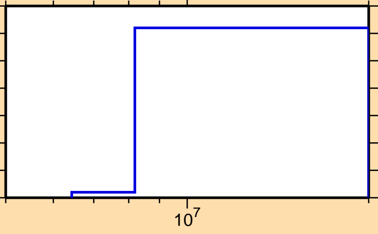
\sigma vs. E for ^{198}\text{Pb}(n,np)
