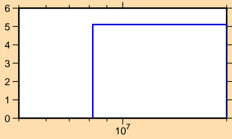
\Delta\sigma/\sigma vs. E for ^{198}\text{Pb}(n,\text{el.})
