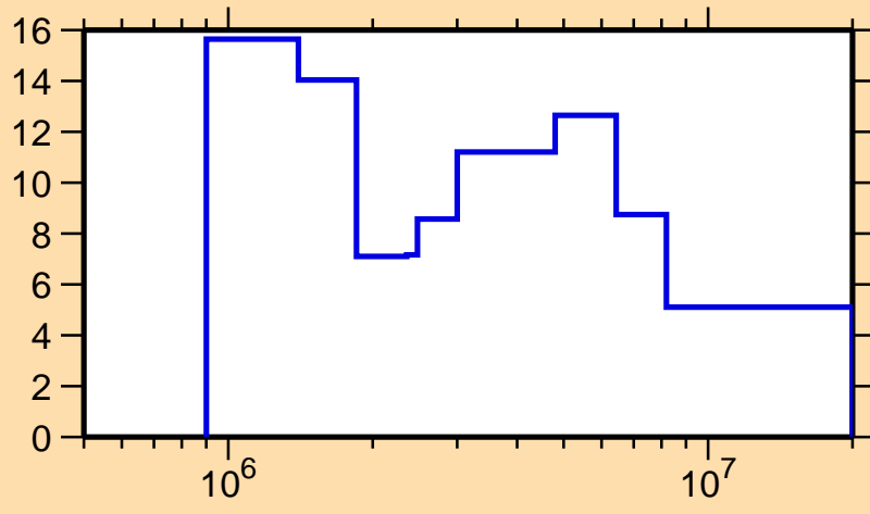
\Delta\sigma/\sigma vs. E for ^{198}\text{Pb}(n,\text{el.})
