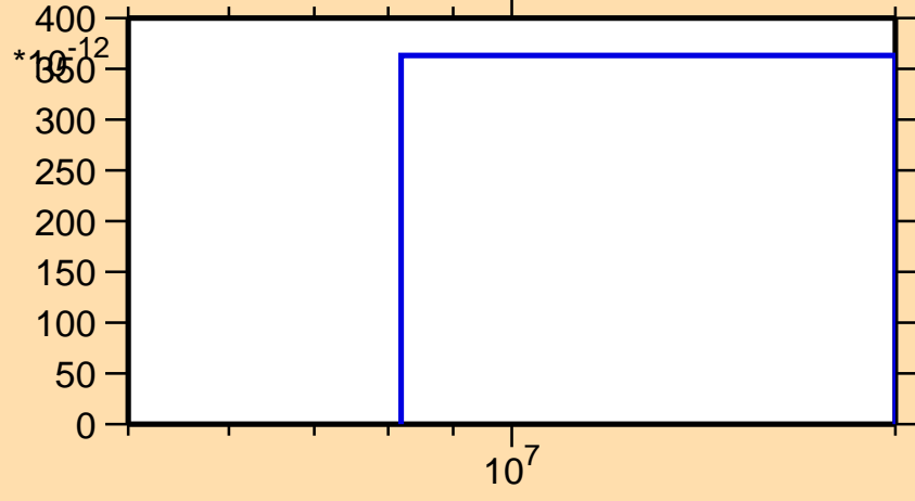
\sigma vs. E for ^{198}\text{Pb}(n,nd)
