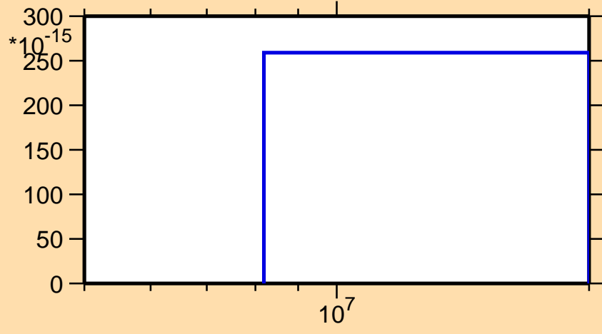
\sigma vs. E for ^{198}\text{Pb}(n,pd)
