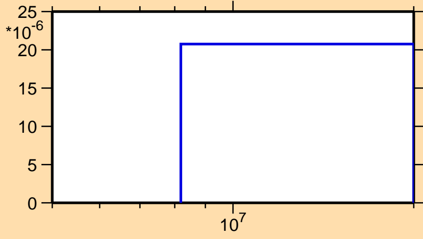
\sigma vs. E for ^{198}\text{Pb}(n,3n)
