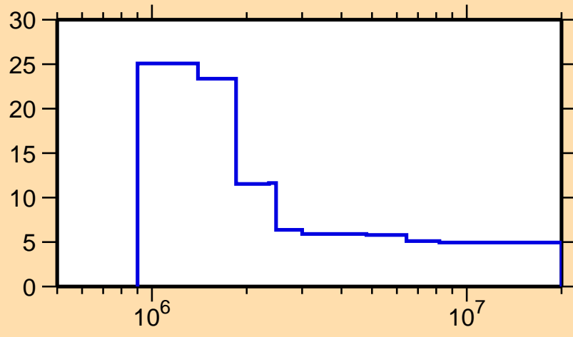
\Delta\sigma/\sigma vs. E for ^{198}\text{Pb}(n,\text{nonel.})
