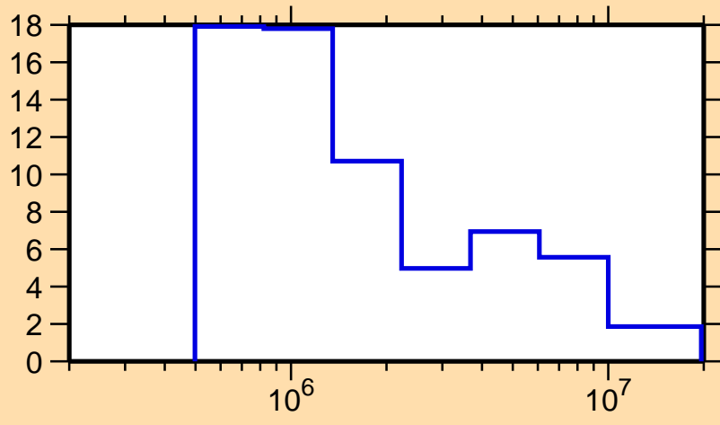
\Delta\sigma/\sigma vs. E for ^{199}\text{Pb}(n, tot.)
