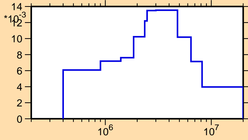
\sigma vs. E for ^{199}\text{Pb}(n,n_2)
