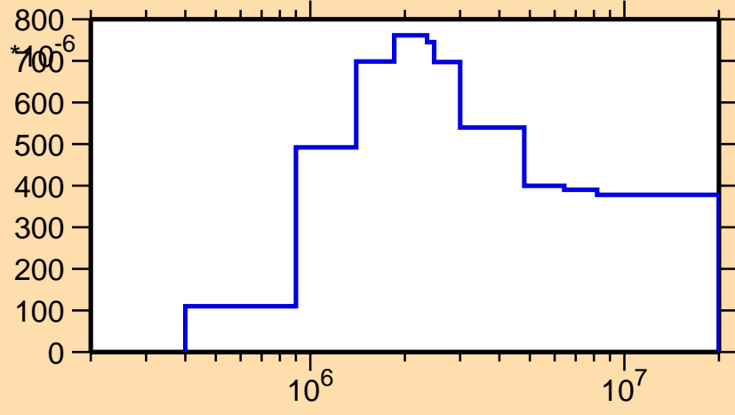
\sigma vs. E for ^{199}\text{Pb}(n,n_1)
