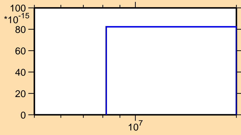
\sigma vs. E for ^{199}\text{Pb}(n,pd)
