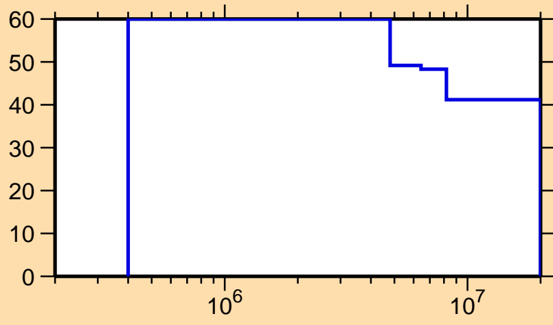
\Delta\sigma/\sigma vs. E for ^{199}\text{Pb}(n,n_1)
