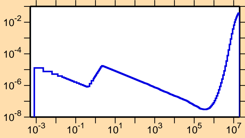
\sigma vs. E for ^{199}\text{Pb}(n,p)
