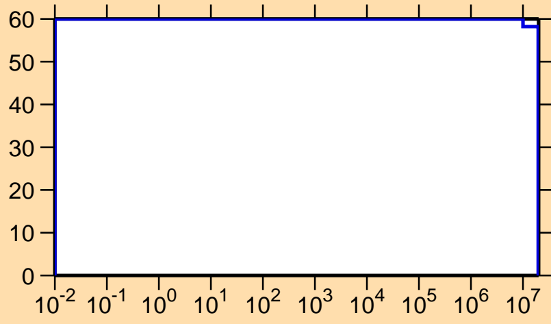
\Delta\sigma/\sigma vs. E for ^{199}\text{Pb}(n,p)
