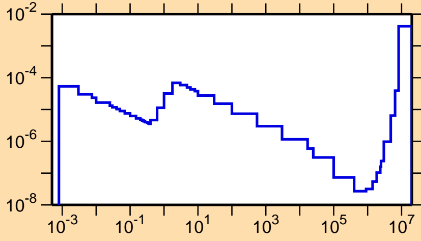
\sigma vs. E for ^{199}\text{Pb}(n,\alpha)
