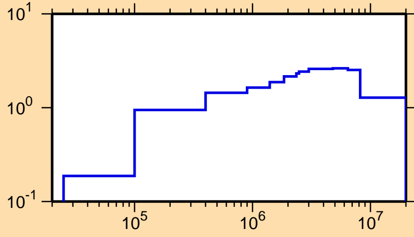
\sigma vs. E for ^{199}\text{Pb}(n,n\text{cont.})
