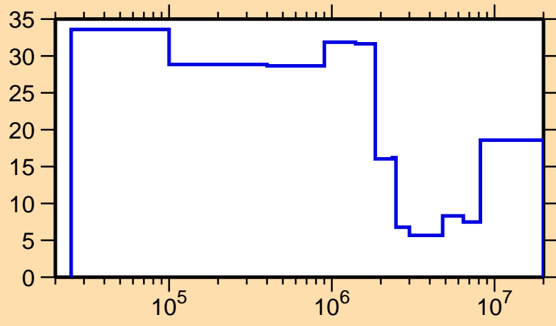
\Delta\sigma/\sigma vs. E for ^{199}\text{Pb}(n,n\text{cont.})
