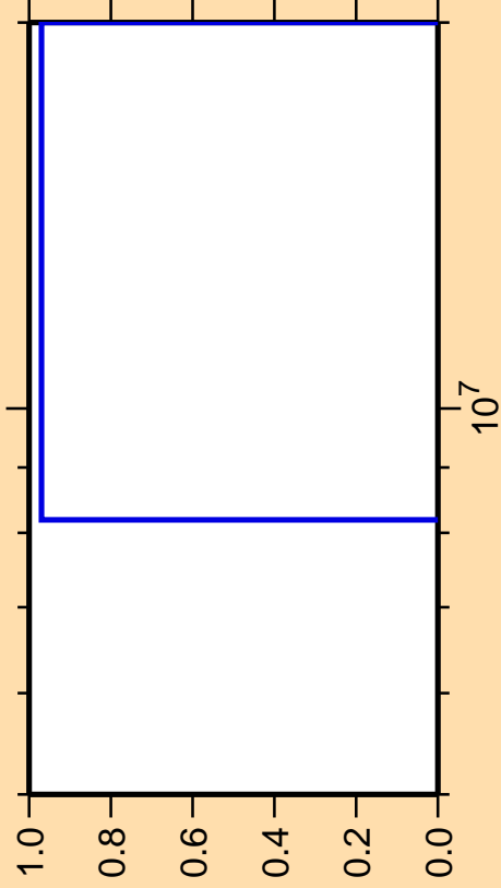
\Delta\sigma/\sigma vs. E for ^{199}\text{Pb}(n,pd)
