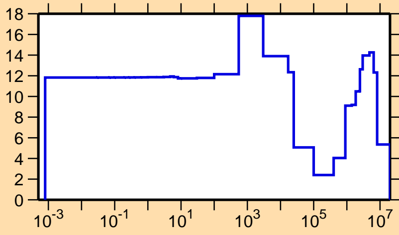
\Delta\sigma/\sigma vs. E for ^{199}\text{Pb}(n,\text{el.})
