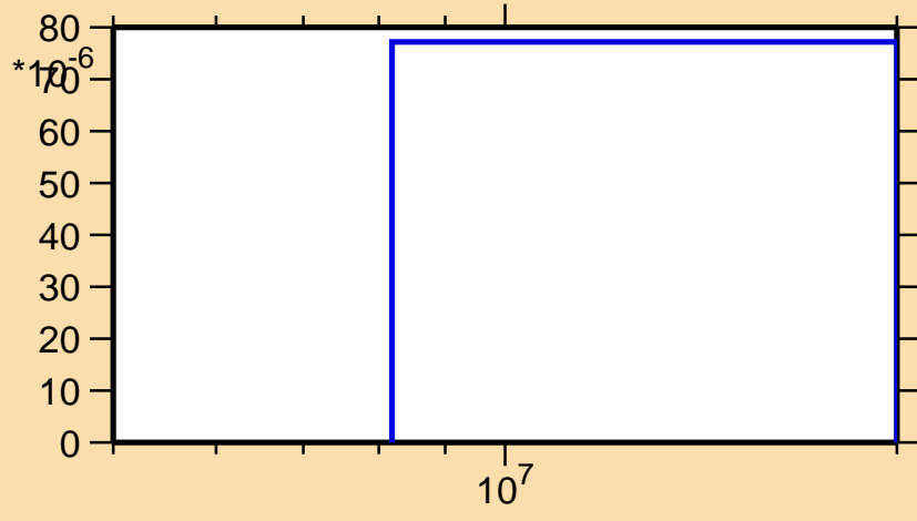
\sigma vs. E for ^{199}\text{Pb}(n,t)
