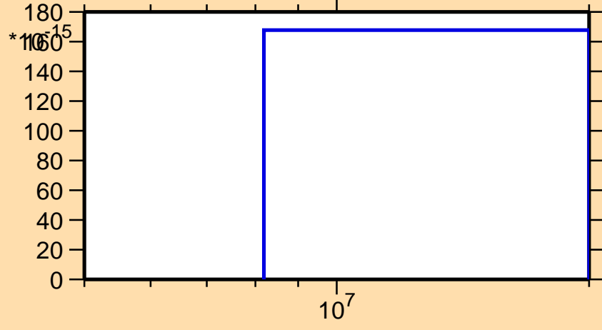
\sigma vs. E for ^{199}\text{Pb}(n,pd)
