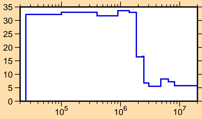
\Delta\sigma/\sigma vs. E for ^{199}\text{Pb}(n,\text{nonel.})
