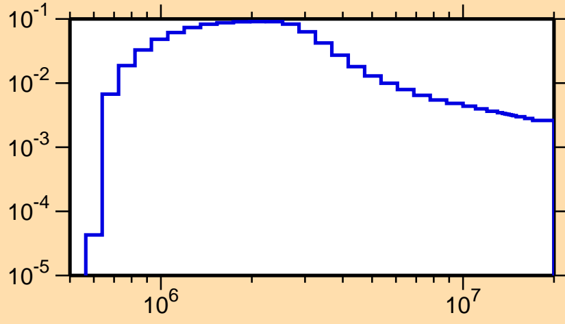
\sigma vs. E for ^{201}\text{Pb}(n,n_4)
