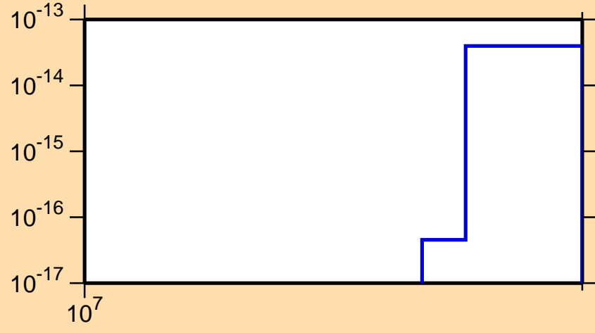
\sigma vs. E for ^{201}\text{Pb}(n,\text{pt})
