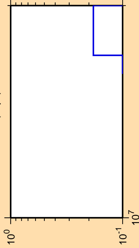
\Delta\sigma/\sigma vs. E for ^{201}\text{Pb}(n,\text{pt})
