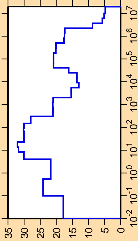
\Delta\sigma/\sigma vs. E for ^{201}\text{Pb}(n,\text{nonel.})
