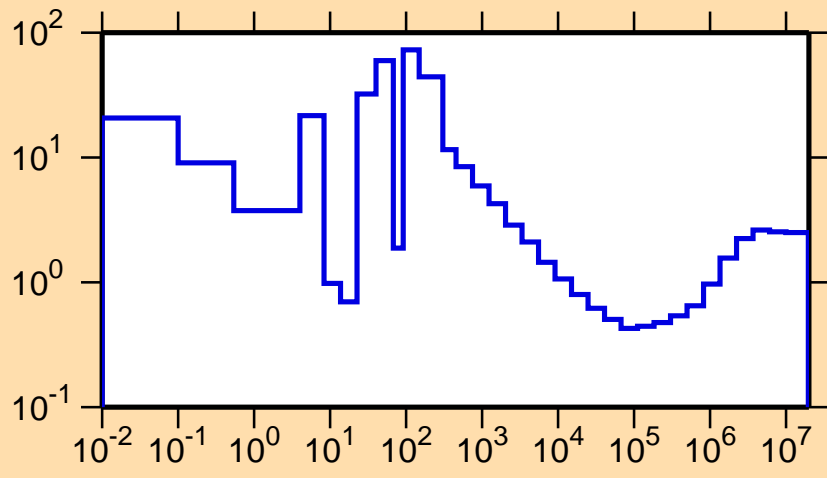
\sigma vs. E for ^{201}\text{Pb}(n,\text{nonel.})
