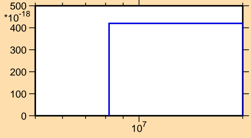
\sigma vs. E for ^{201}\text{Pb}(\text{mt } 34)
