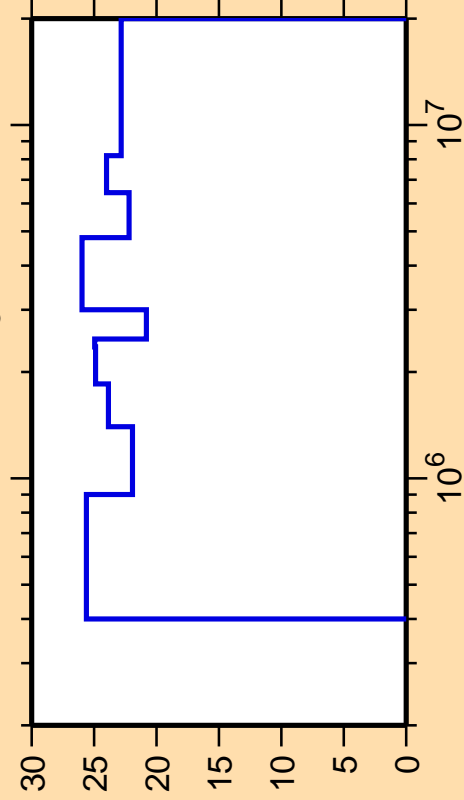
\Delta\sigma/\sigma vs. E for ^{201}\text{Pb}(n,n_3)
