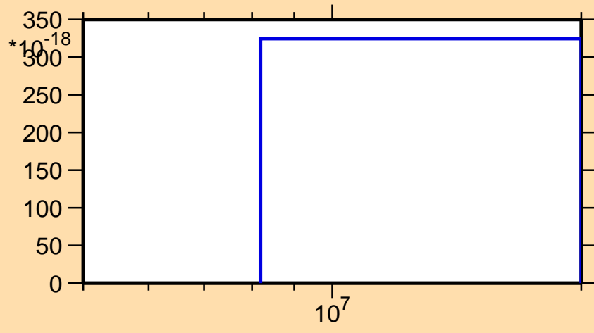
\sigma vs. E for ^{201}\text{Pb}(n,\text{pt})
