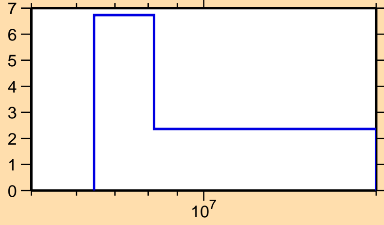
\Delta\sigma/\sigma vs. E for ^{201}\text{Pb}(n,\text{el.})
