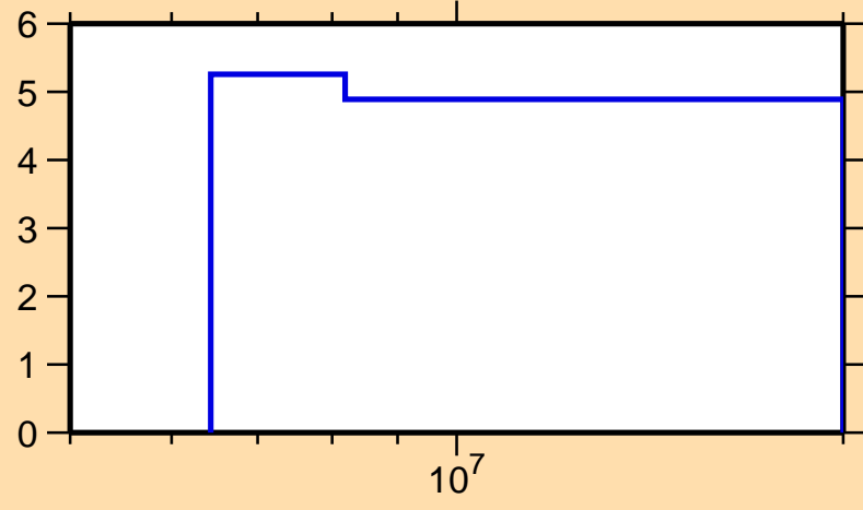
\Delta\sigma/\sigma vs. E for ^{201}\text{Pb}(n,\text{nonel.})
