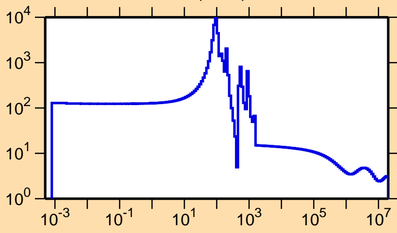
\sigma vs. E for ^{202}\text{Pb}(n,\text{el.})
