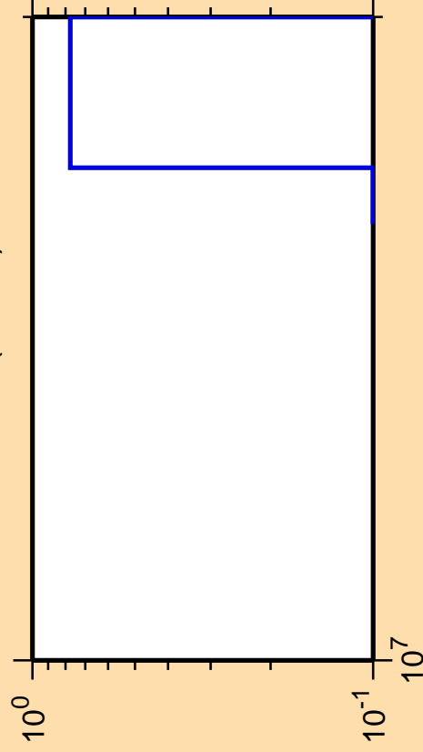
\Delta\sigma/\sigma vs. E for ^{202}\text{Pb} (mt 34)
