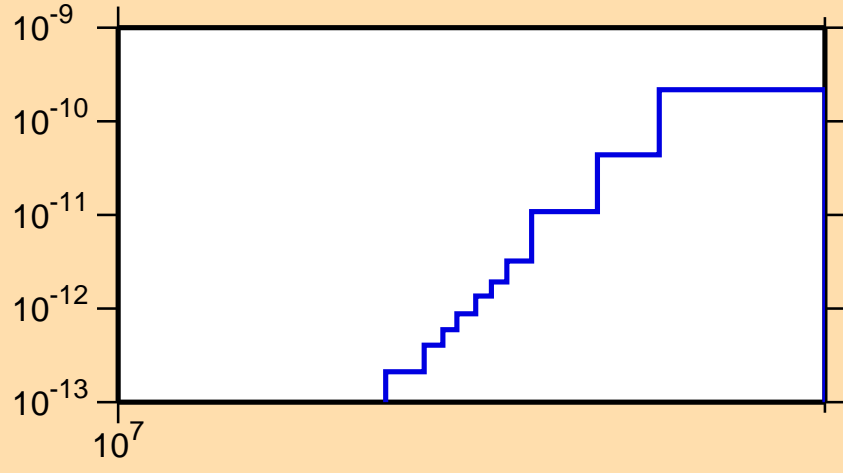
\sigma vs. E for ^{202}\text{Pb}(n,p\alpha)
