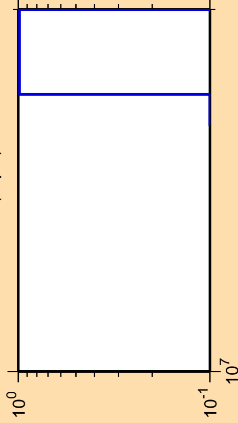
\Delta\sigma/\sigma vs. E for ^{202}\text{Pb}(n,\text{pd})
