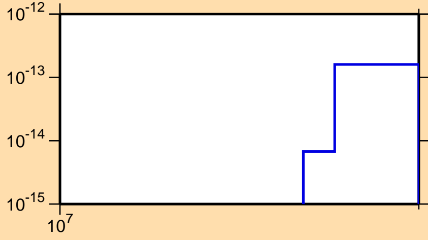
\sigma vs. E for ^{202}\text{Pb}(n,\text{pd})
