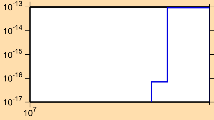
\sigma vs. E for ^{202}\text{Pb} (mt 34)
