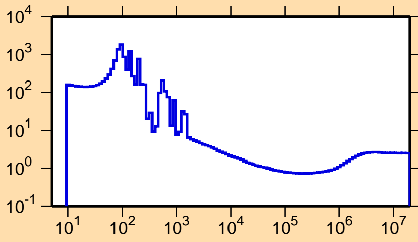
\sigma vs. E for ^{202}\text{Pb}(n,\text{nonel.})
