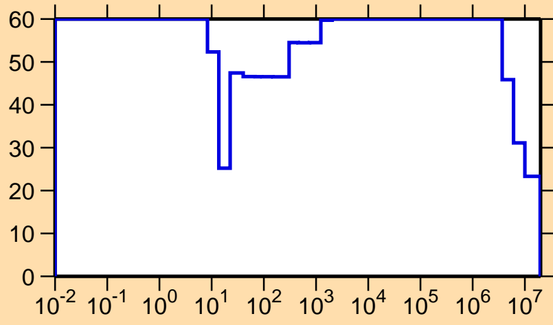
\Delta\sigma/\sigma vs. E for ^{202}\text{Pb}(n,p)
