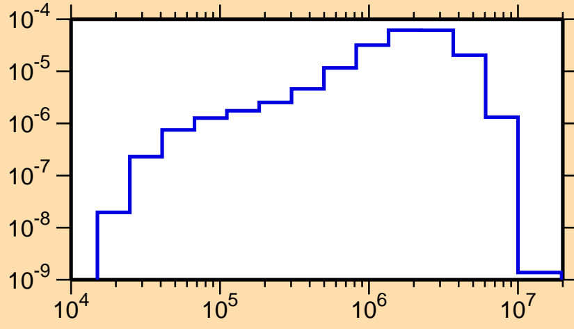
\sigma vs. E for ^{202}\text{Pb}(n,n_1)
