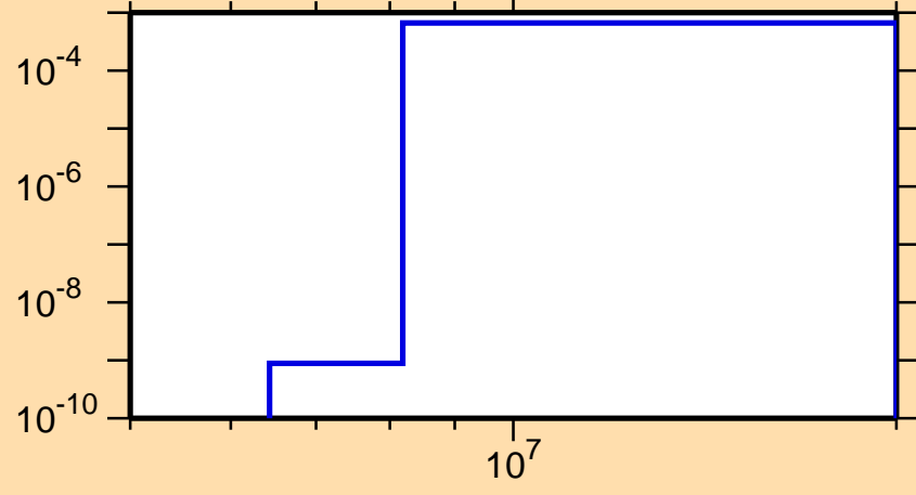
\sigma vs. E for ^{202}\text{Pb}(n,np)
