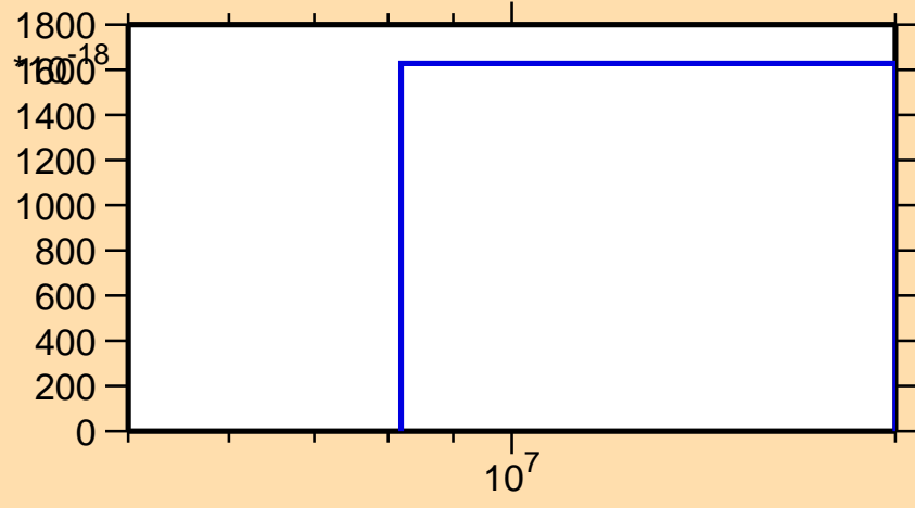
\sigma vs. E for ^{202}\text{Pb}(n,pd)
