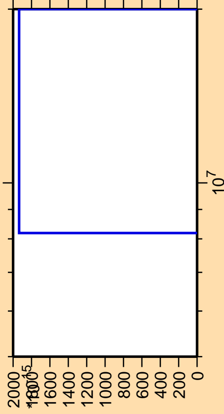
\Delta\sigma/\sigma vs. E for ^{202}\text{Pb}(\text{mt } 42)
