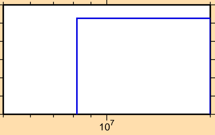
\sigma vs. E for ^{202}\text{Pb}(n,2n\alpha)
