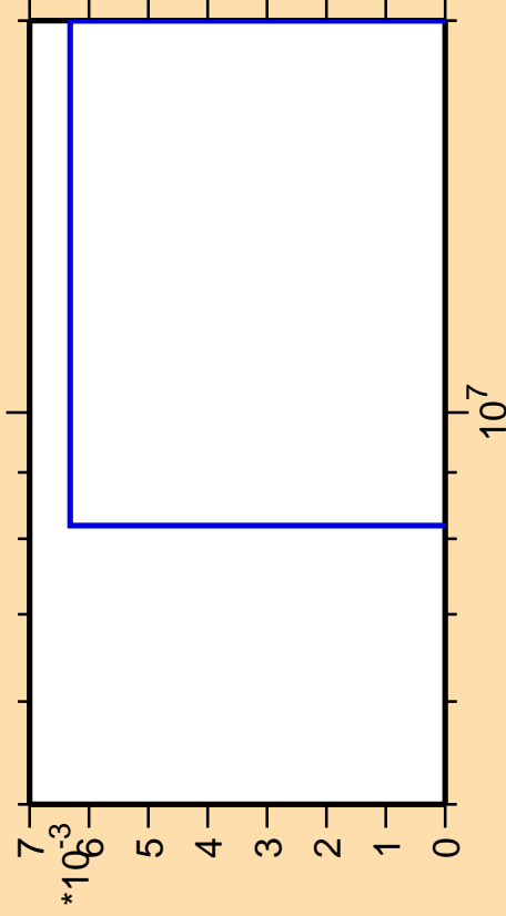
\Delta\sigma/\sigma vs. E for ^{202}\text{Pb} (mt 34)
