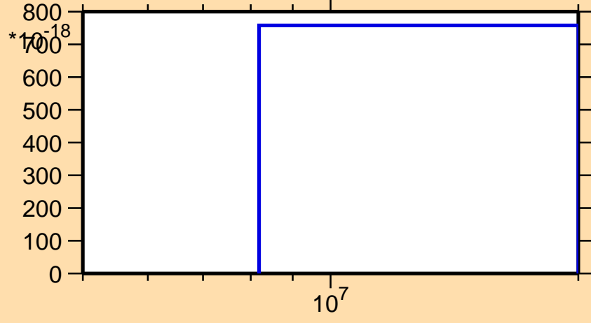
\sigma vs. E for ^{202}\text{Pb} (mt 34)
