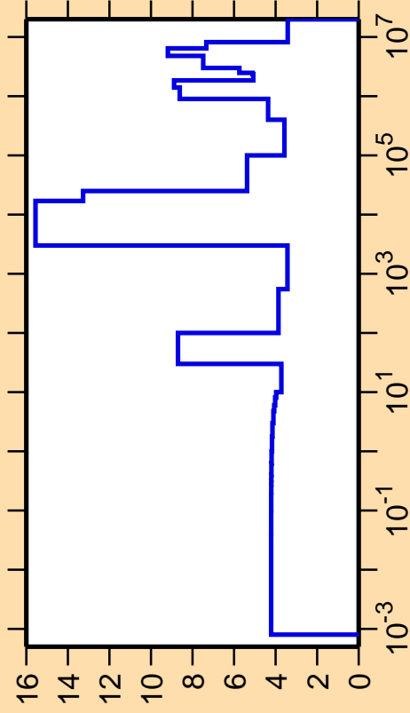
\Delta\sigma/\sigma vs. E for ^{202}\text{Pb}(n,\text{el.})
