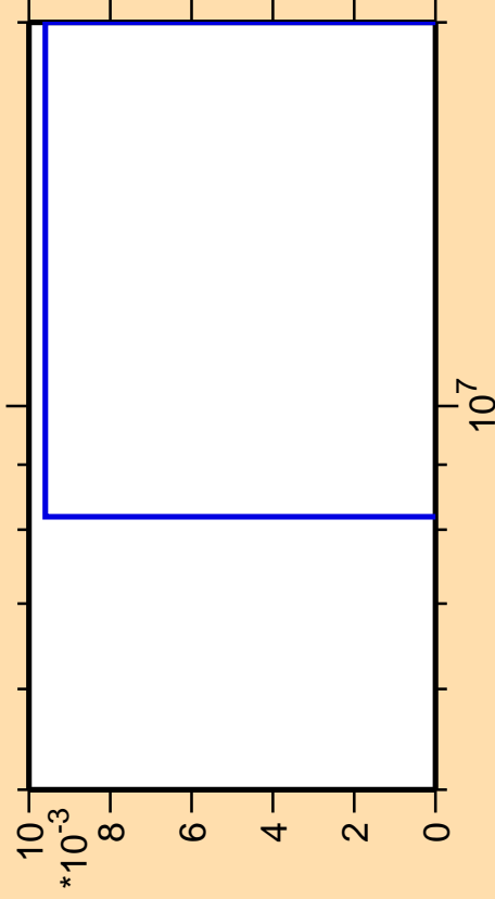
\Delta\sigma/\sigma vs. E for ^{202}\text{Pb}(n,pd)
