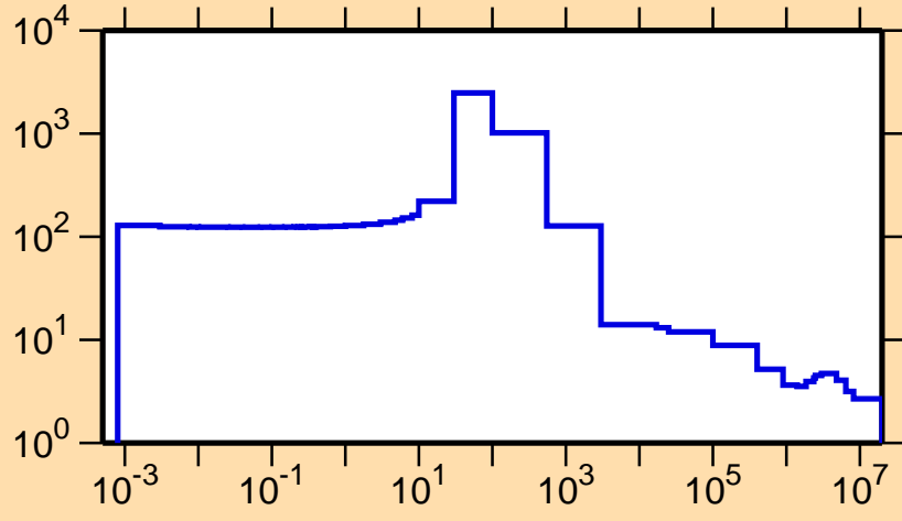
\sigma vs. E for ^{202}\text{Pb}(n,\text{el.})
