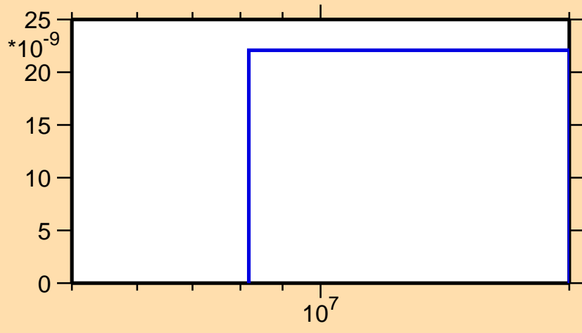
\sigma vs. E for ^{202}\text{Pb}(n,2np)
