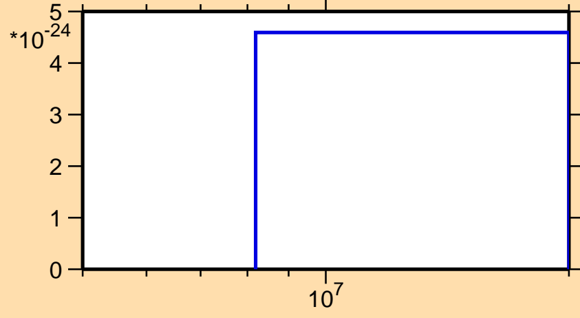
\sigma vs. E for ^{202}\text{Pb}(\text{mt } 42)
