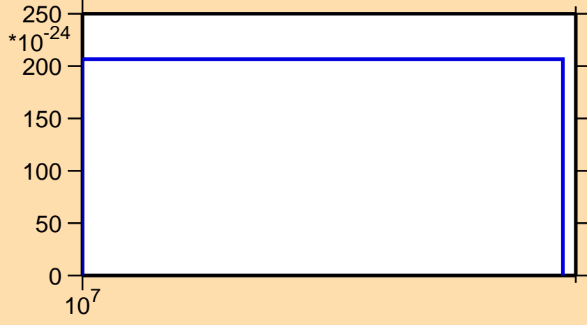
\sigma vs. E for ^{203}\text{Pb} (mt 11)
