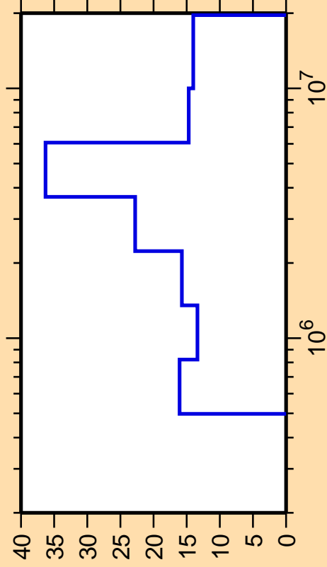
\Delta\sigma/\sigma vs. E for ^{203}\text{Pb}(n,n_3)
