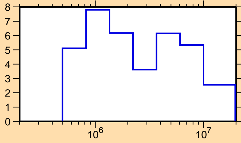
\Delta\sigma/\sigma vs. E for ^{203}\text{Pb}(n,\text{el.})
