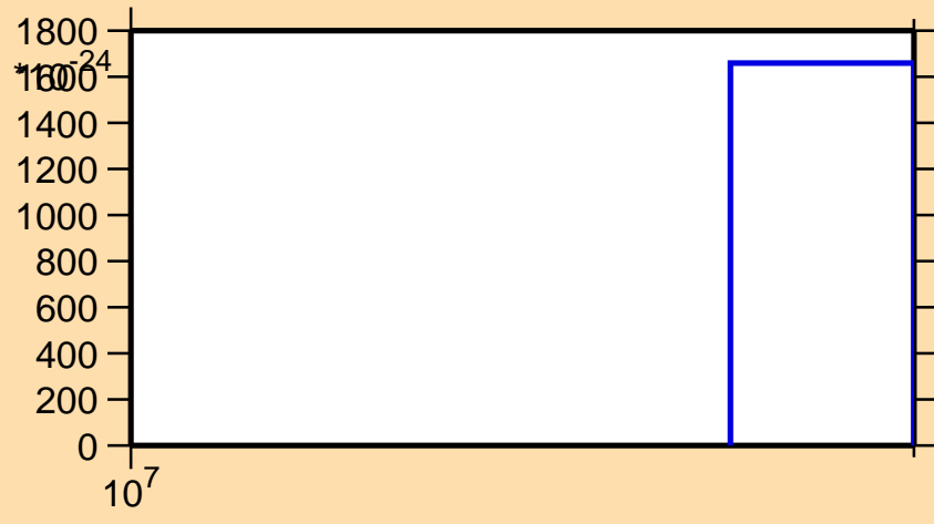
\sigma vs. E for ^{204}\text{Pb} (mt 11)
