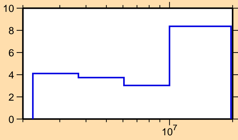
\Delta\sigma/\sigma vs. E for ^{204}\text{Pb}(n,n\text{cont.})
