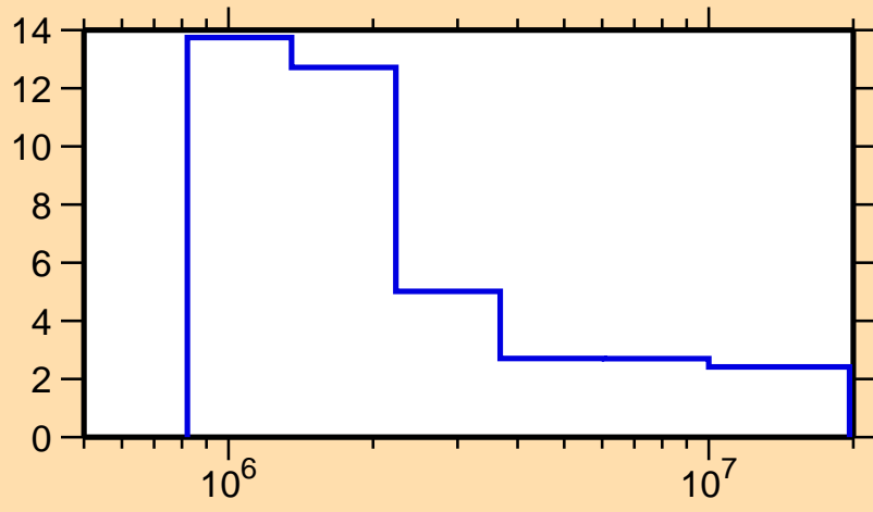
\Delta\sigma/\sigma vs. E for ^{204}\text{Pb}(n,\text{nonel.})
