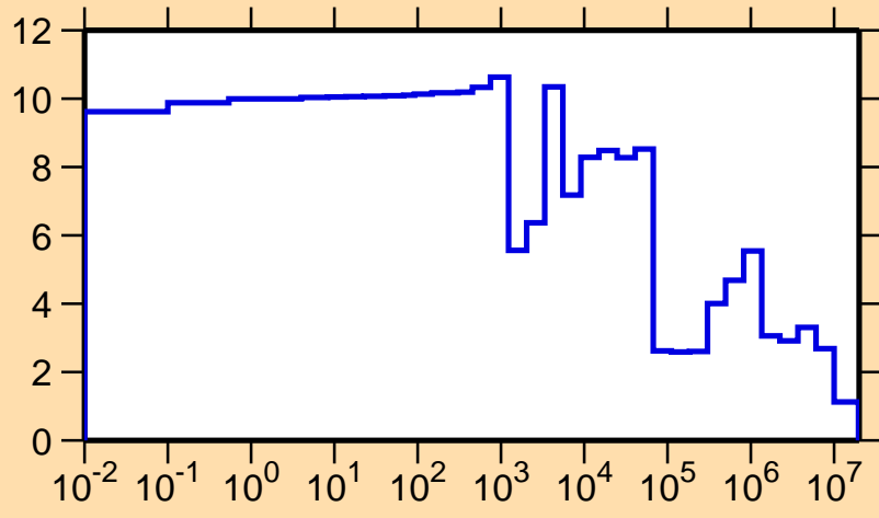
\Delta\sigma/\sigma vs. E for ^{204}\text{Pb}(n,\text{tot.})
