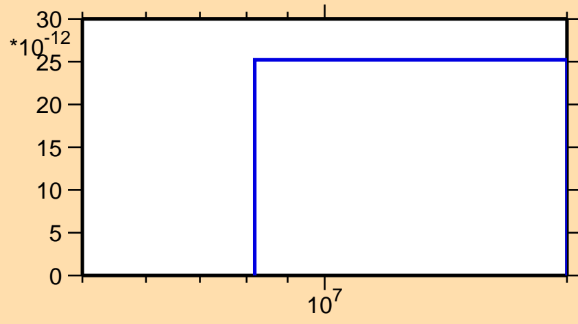
\sigma vs. E for ^{204}\text{Pb}(n,2n\alpha)
