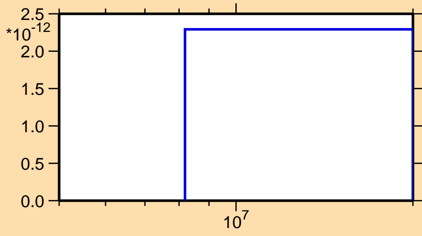
\sigma vs. E for ^{204}\text{Pb}(n,\text{He}3)
