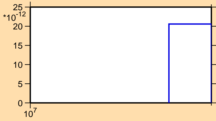
\sigma vs. E for ^{204}\text{Pb}(\text{mt117})
