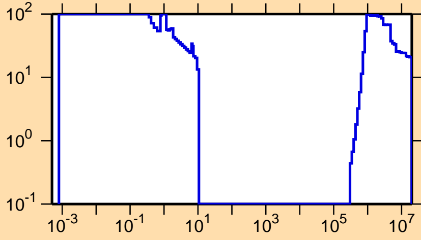
\Delta\sigma/\sigma vs. E for ^{204}\text{Pb}(n,p)
