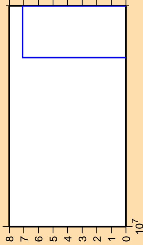
\Delta\sigma/\sigma vs. E for ^{204}\text{Pb} (mt 45)
