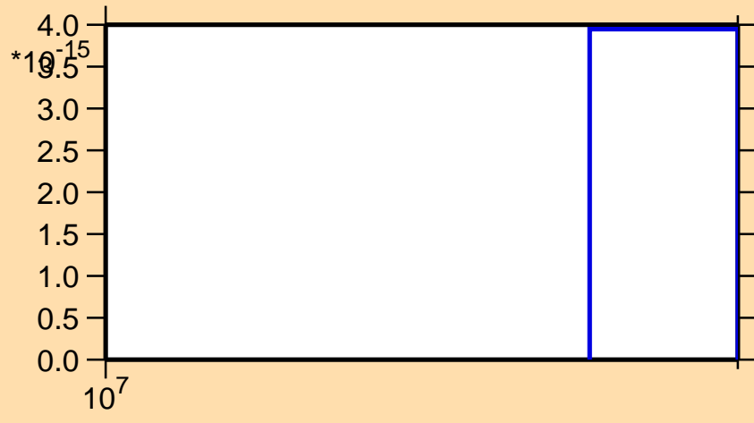
\sigma vs. E for ^{204}\text{Pb} (mt 34)
