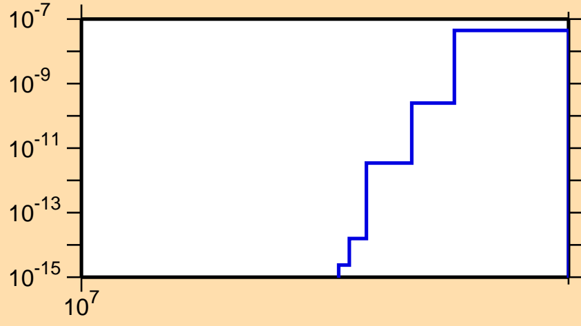
\sigma vs. E for ^{204}\text{Pb}(n,nt)
