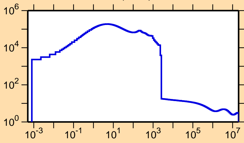
\sigma vs. E for ^{204}\text{Pb}(n,\text{el.})
