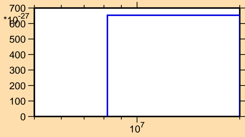
\sigma vs. E for ^{204}\text{Pb} (mt 42)
