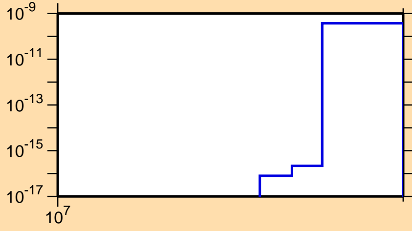
\sigma vs. E for ^{206}\text{Pb}(n,2np)
