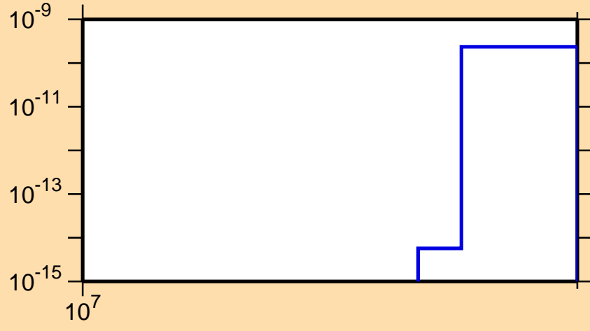
\sigma vs. E for ^{206}\text{Pb}(n,nt)
