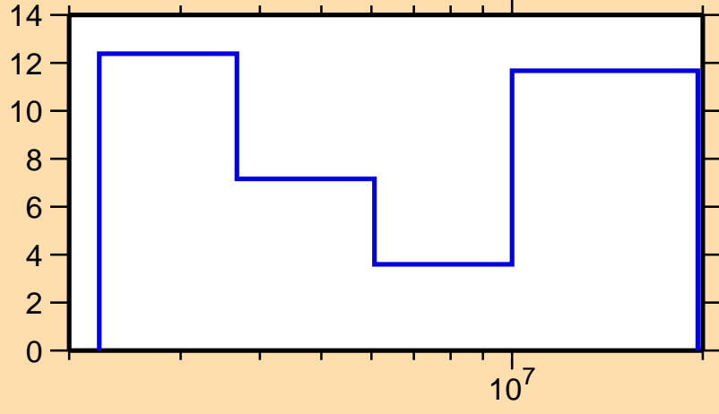
\Delta\sigma/\sigma vs. E for ^{206}\text{Pb}(n,n\text{cont.})
