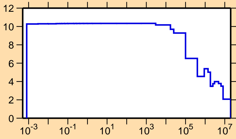
\Delta\sigma/\sigma vs. E for ^{206}\text{Pb}(n,\text{tot.})
