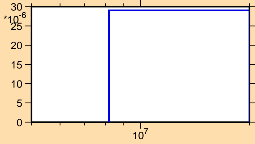
\sigma vs. E for ^{206}\text{Pb}(n,np)
