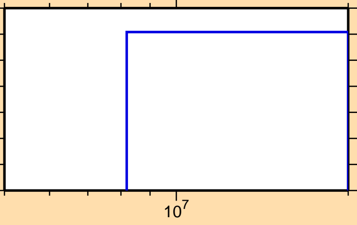
\sigma vs. E for ^{206}\text{Pb}(n,2np)
