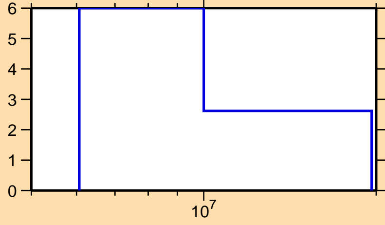
\Delta\sigma/\sigma vs. E for ^{207}\text{Pb}(n,2n)
