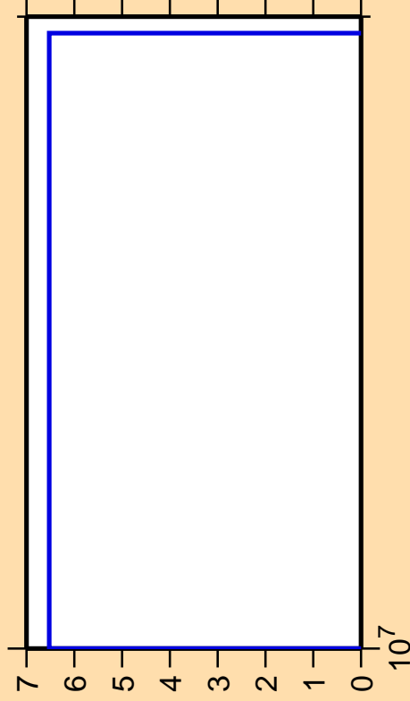
\Delta\sigma/\sigma vs. E for ^{207}\text{Pb}(n,nt)
