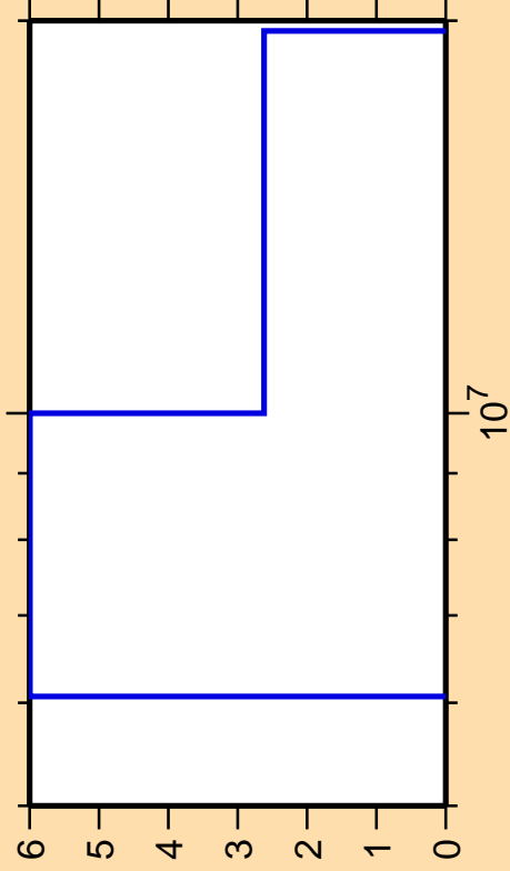
\Delta\sigma/\sigma vs. E for ^{207}\text{Pb}(n,2n)
