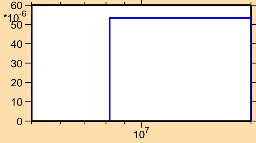
\sigma vs. E for ^{207}\text{Pb}(n,d)
