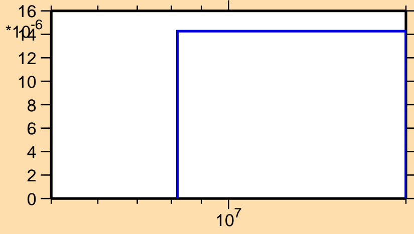
\sigma vs. E for ^{207}\text{Pb}(n,np)
