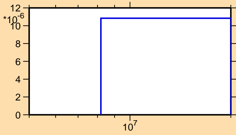
\sigma vs. E for ^{207}\text{Pb}(n,t)
