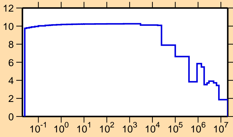
\Delta\sigma/\sigma vs. E for ^{207}\text{Pb}(n,\text{tot.})
