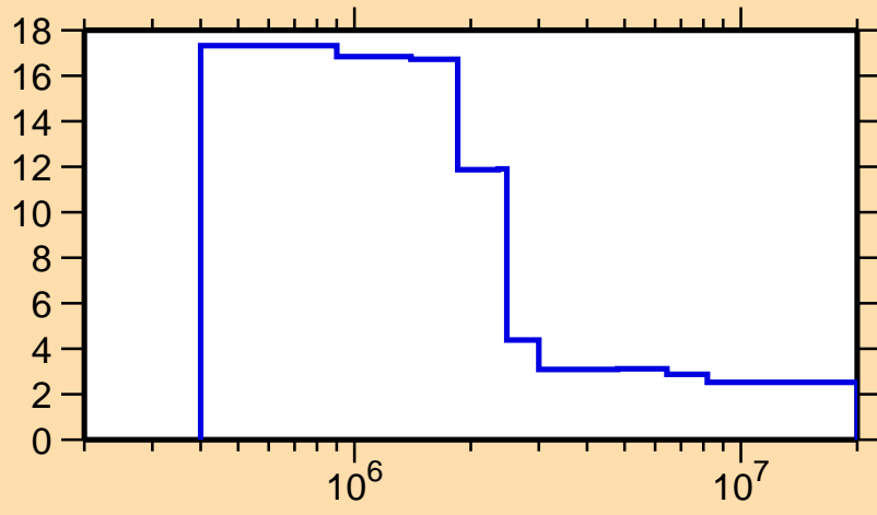
\Delta\sigma/\sigma vs. E for ^{207}\text{Pb}(n,\text{nonel.})
