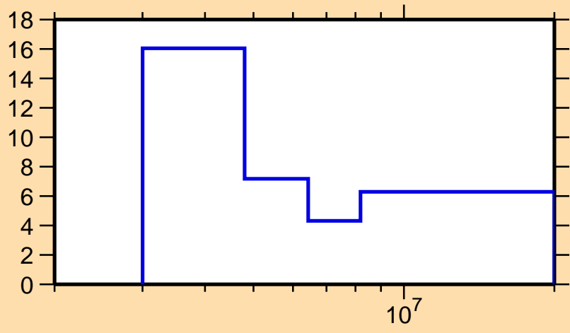
\Delta\sigma/\sigma vs. E for ^{207}\text{Pb}(n,n\text{cont.})
