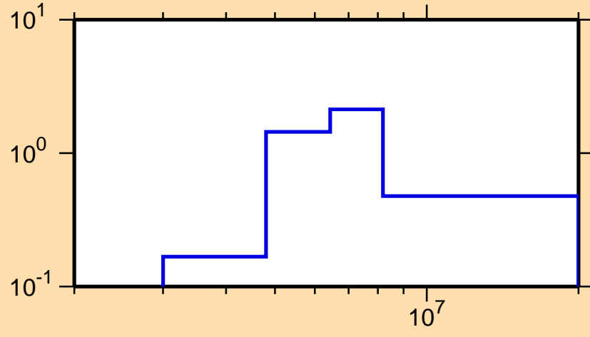
\sigma vs. E for ^{207}\text{Pb}(n,n\text{cont.})
