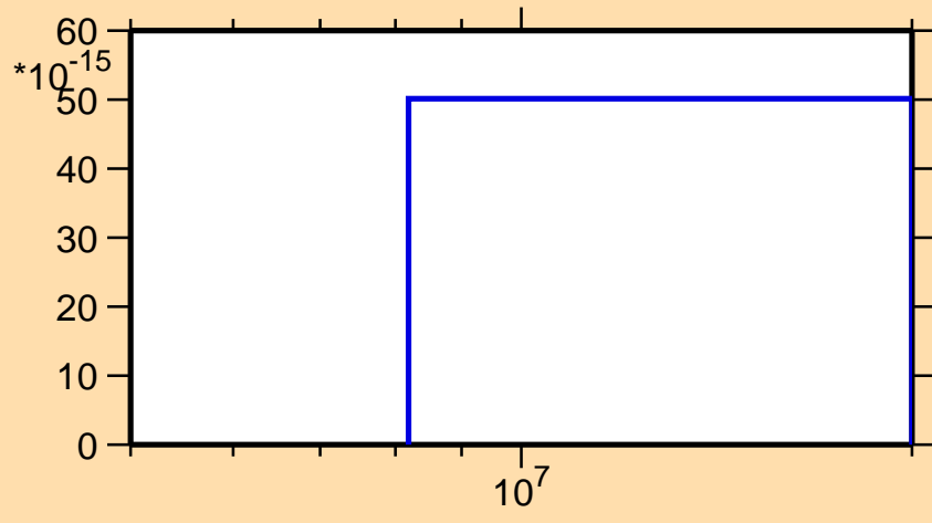
\sigma vs. E for ^{207}\text{Pb}(n,\text{He}3)
