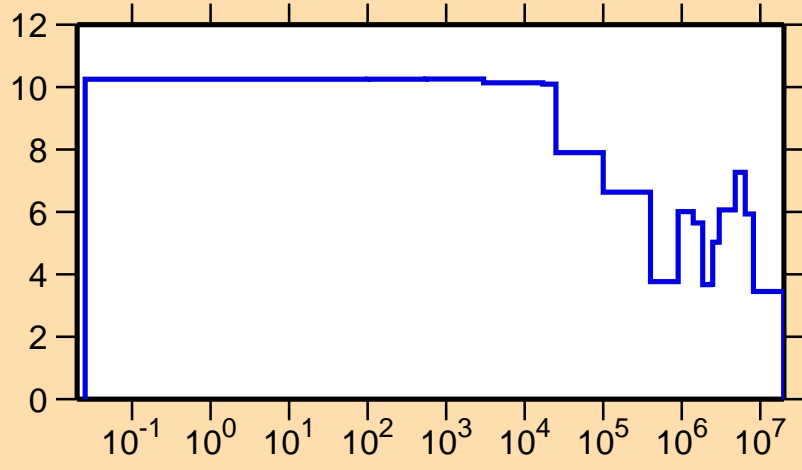
\Delta\sigma/\sigma vs. E for ^{207}\text{Pb}(n,\text{el.})
