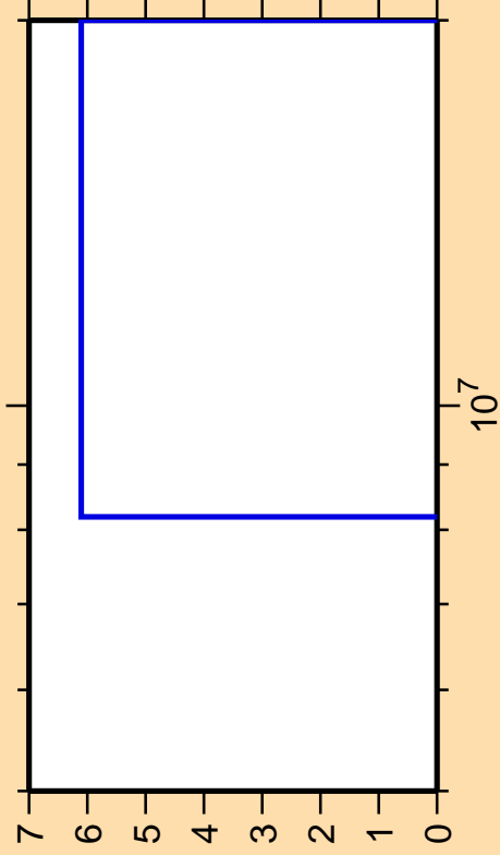
\Delta\sigma/\sigma vs. E for ^{207}\text{Pb}(n,3n)
