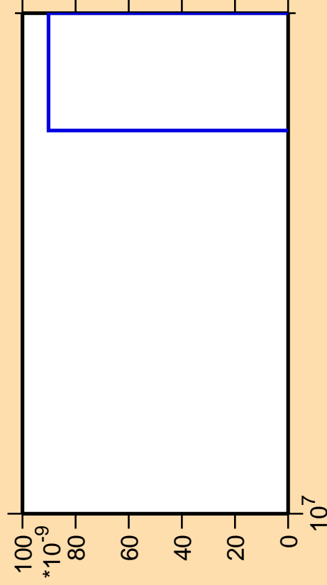
\Delta\sigma/\sigma vs. E for ^{209}\text{Pb}(\text{mt } 42)
