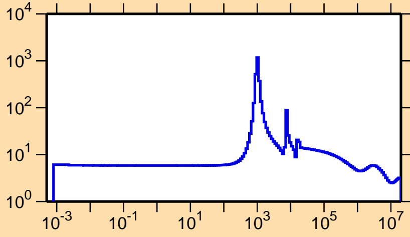
\sigma vs. E for ^{209}\text{Pb}(n,\text{el.})
