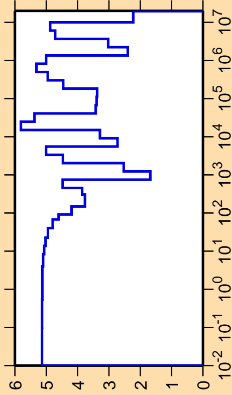
\Delta\sigma/\sigma vs. E for ^{209}\text{Pb}(n,\text{el.})
