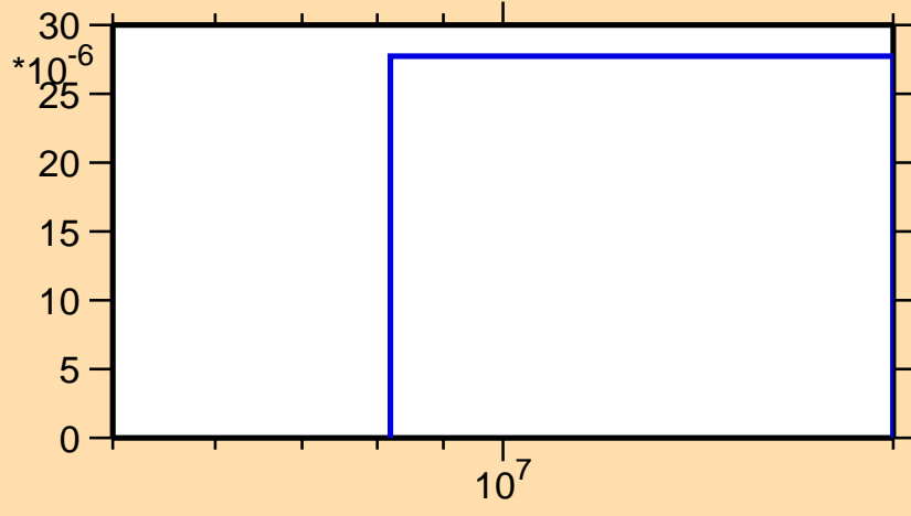
\sigma vs. E for ^{210}\text{Pb}(n,t)
