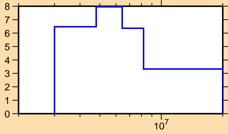
\Delta\sigma/\sigma vs. E for ^{210}\text{Pb}(n,\text{el.})
