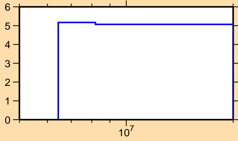
\Delta\sigma/\sigma vs. E for ^{210}\text{Pb}(n,2n)
