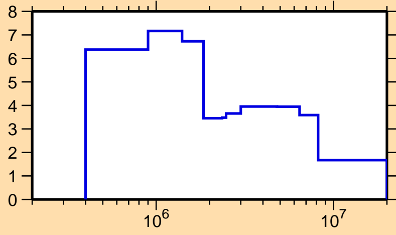
\Delta\sigma/\sigma vs. E for ^{210}\text{Pb}(n,\text{tot.})
