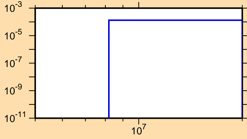
\sigma vs. E for ^{210}\text{Pb}(n,p)
