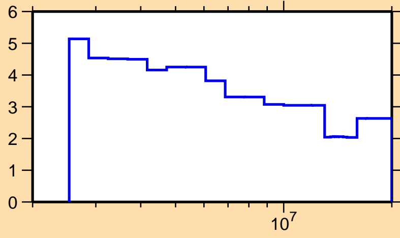
\Delta\sigma/\sigma vs. E for ^{211}\text{Pb}(n,\text{nonel.})
