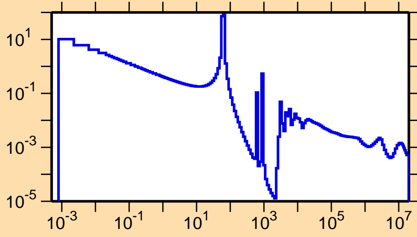
\sigma vs. E for ^{211}\text{Pb}(n,\gamma)
