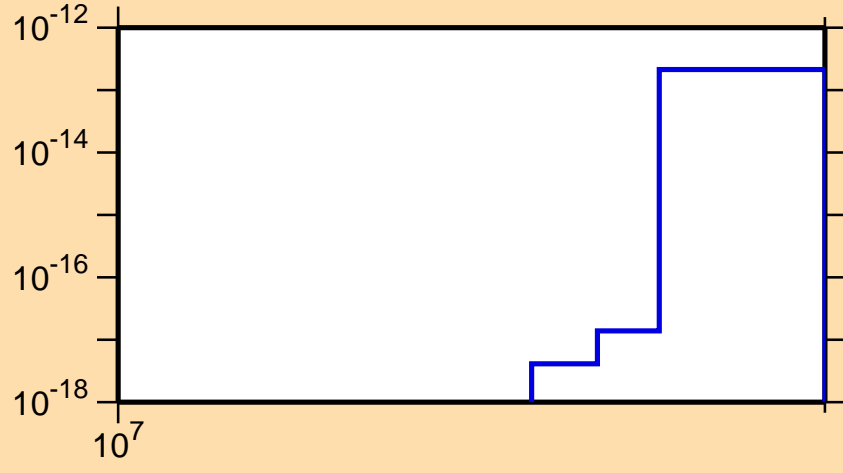
\sigma vs. E for ^{211}\text{Pb} (mt 11)
