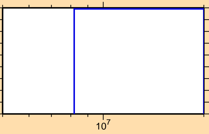
\sigma vs. E for ^{211}\text{Pb}(n,d)
