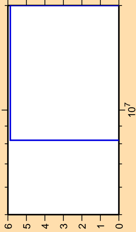
\Delta\sigma/\sigma vs. E for ^{211}\text{Pb}(n,3n)
