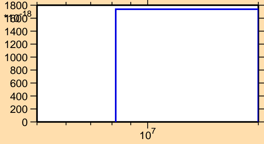
\sigma vs. E for ^{211}\text{Pb}(\text{mt } 11)
