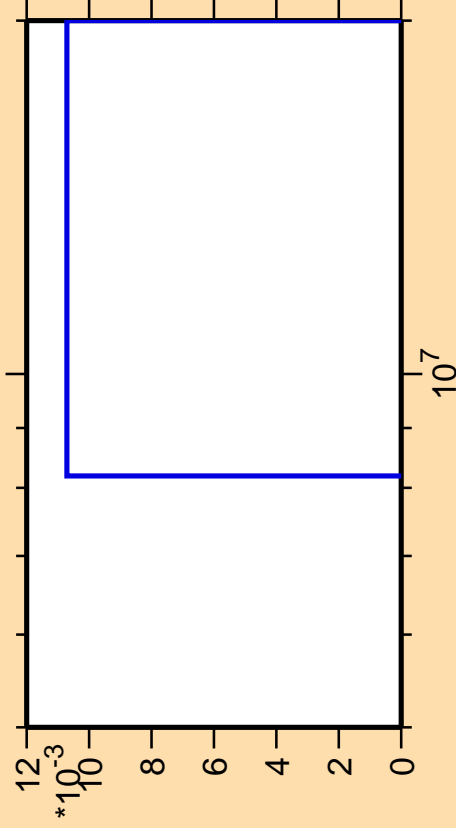
\Delta\sigma/\sigma vs. E for ^{211}\text{Pb}(\text{mt } 11)
