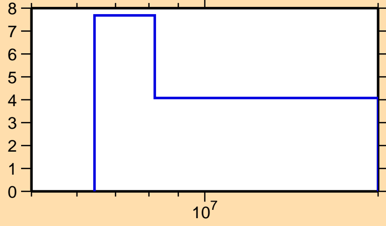
\Delta\sigma/\sigma vs. E for ^{211}\text{Pb}(n,\text{el.})
