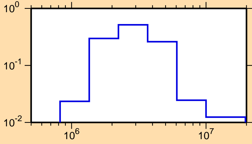
\sigma vs. E for ^{212}\text{Pb}(n,n_2)
