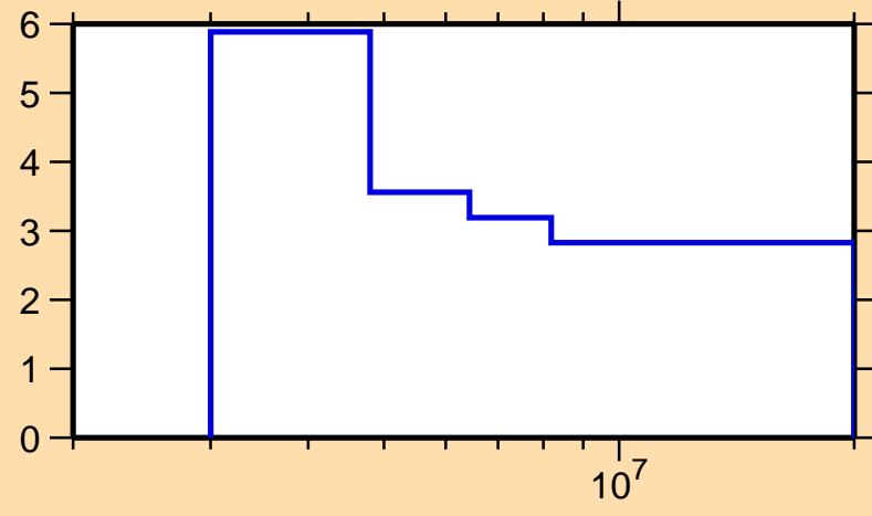
\Delta\sigma/\sigma vs. E for ^{212}\text{Pb}(n,\text{nonel.})
