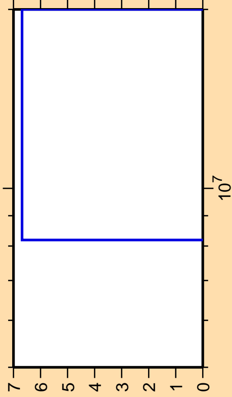
\Delta\sigma/\sigma vs. E for ^{212}\text{Pb}(n,3n)
