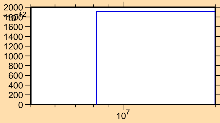
\sigma vs. E for ^{212}\text{Pb}(n,\text{nd})
