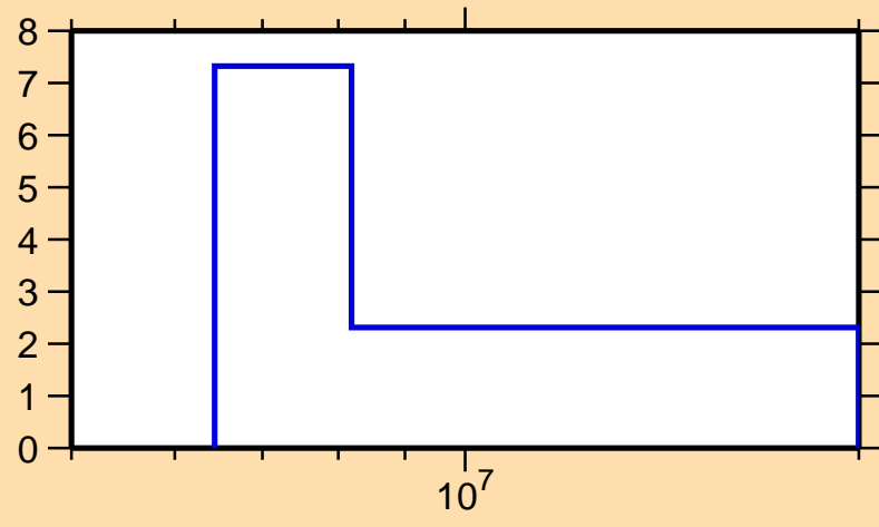
\Delta\sigma/\sigma vs. E for ^{212}\text{Pb}(n,\text{tot.})
