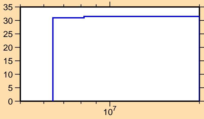
\Delta\sigma/\sigma vs. E for ^{213}\text{Pb}(n,n\text{cont.})
