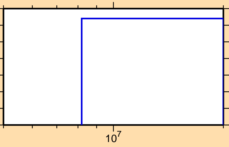
\sigma vs. E for ^{213}\text{Pb}(n,d)
