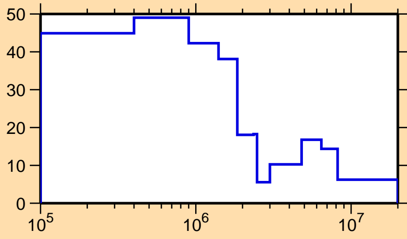
\Delta\sigma/\sigma vs. E for ^{213}\text{Pb}(n, el.)
