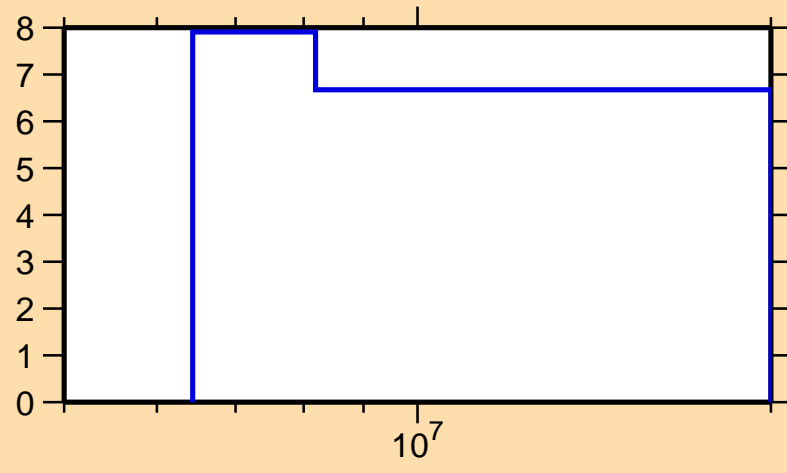
\Delta\sigma/\sigma vs. E for ^{213}\text{Pb}(n,\text{nonel.})
