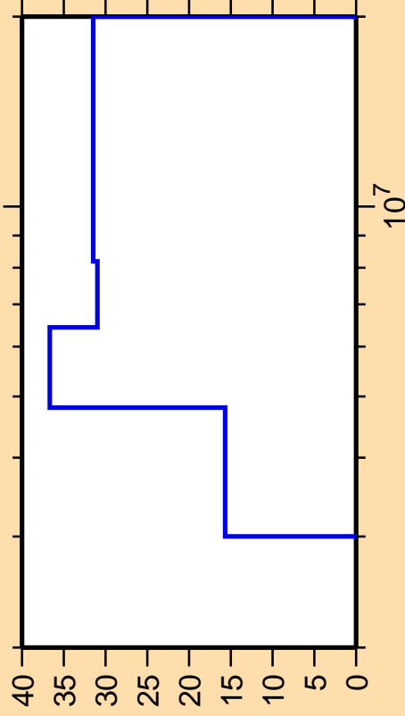
\Delta\sigma/\sigma vs. E for ^{213}\text{Pb}(n,n\text{cont.})
