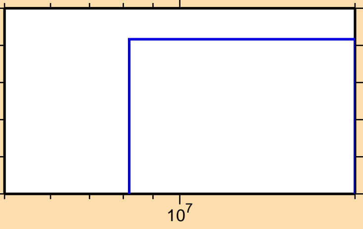
\sigma vs. E for ^{213}\text{Pb}(n,2n\alpha)
