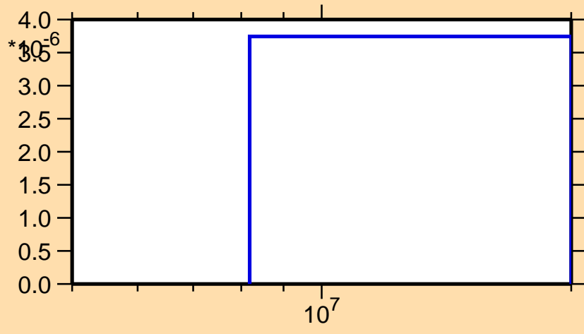
\sigma vs. E for ^{213}\text{Pb}(n,np)
