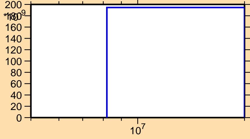
\sigma vs. E for ^{213}\text{Pb}(n,nt)
