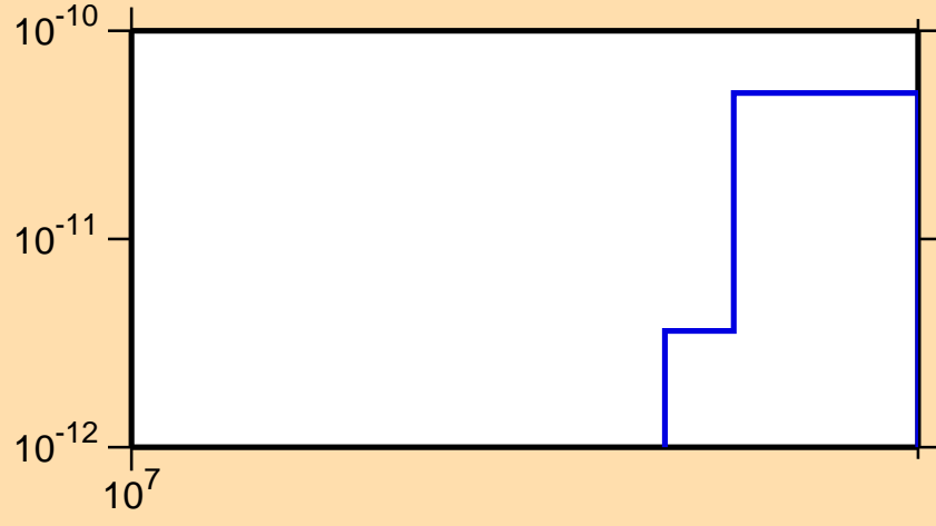
\sigma vs. E for ^{214}\text{Pb}(n,3n\alpha)
