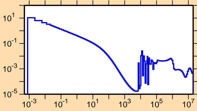
\sigma vs. E for ^{214}\text{Pb}(n,\gamma)
