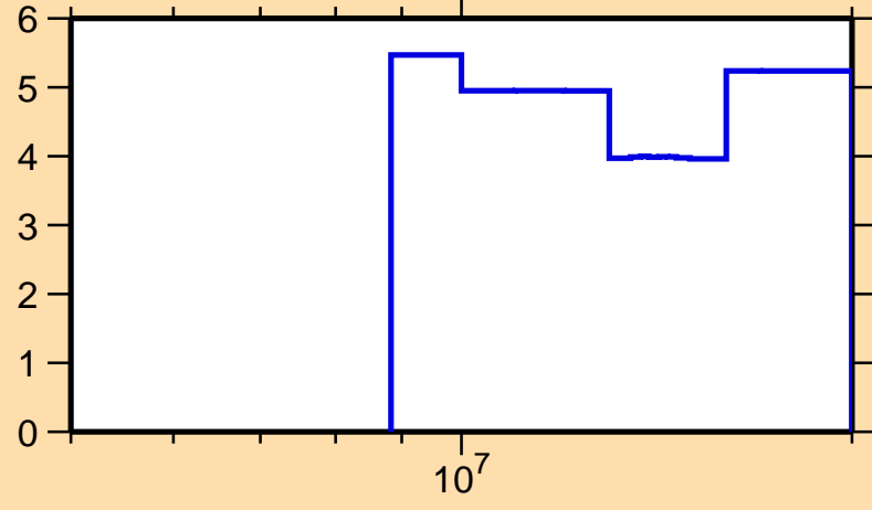
\Delta\sigma/\sigma vs. E for ^{214}\text{Pb}(n,\text{tot.})
