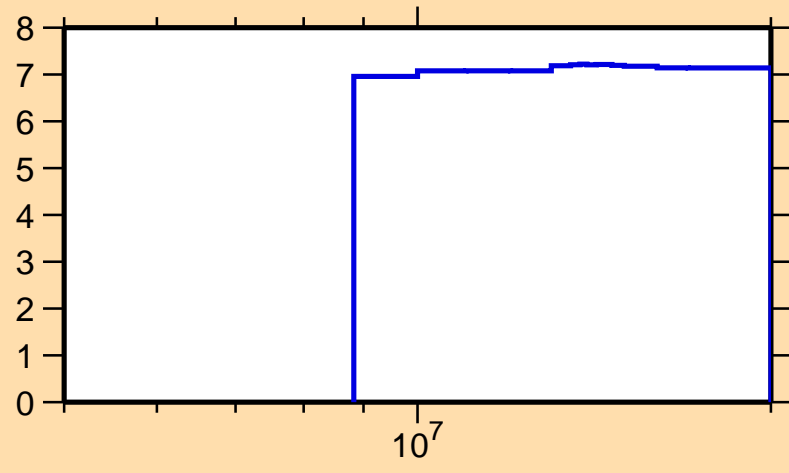
\Delta\sigma/\sigma vs. E for ^{214}\text{Pb}(n,\text{nonel.})
