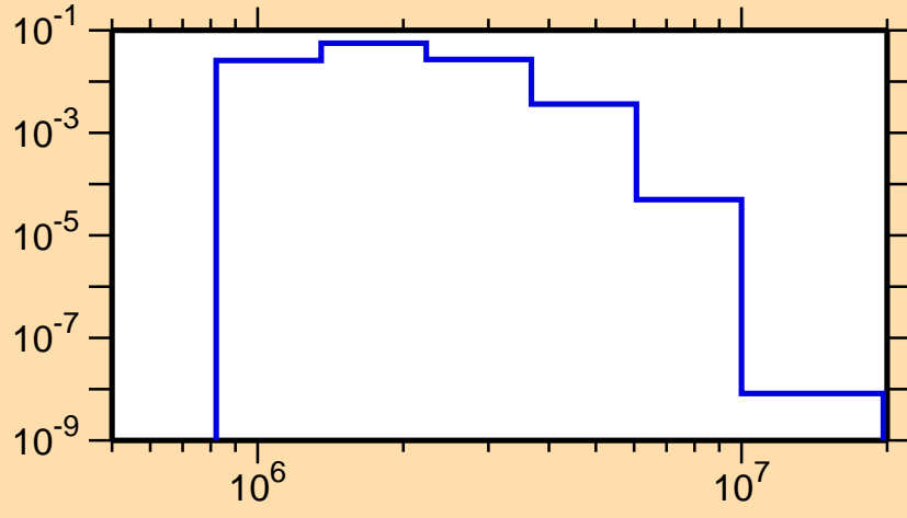
\sigma vs. E for ^{214}\text{Pb}(n,n_3)
