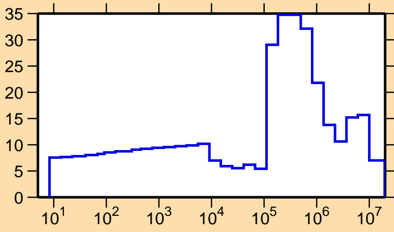
\Delta\sigma/\sigma vs. E for ^{214}\text{Pb}(n,\text{el.})
