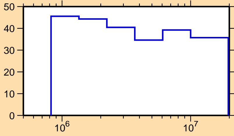
\Delta\sigma/\sigma vs. E for ^{214}\text{Pb}(n,n_1)
