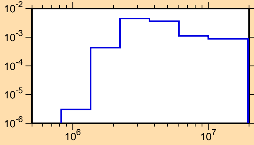
\sigma vs. E for ^{214}\text{Pb}(n,n_4)
