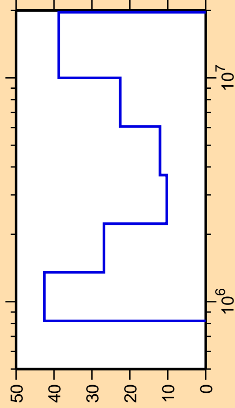
\Delta\sigma/\sigma vs. E for ^{214}\text{Pb}(n,\text{inel.})
