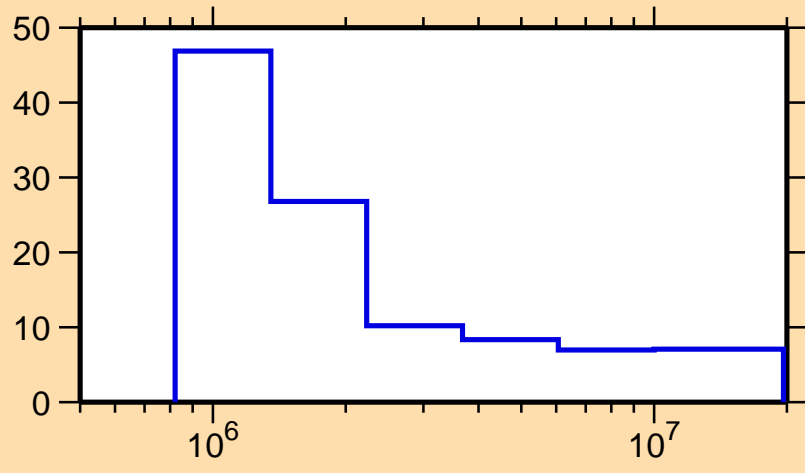
\Delta\sigma/\sigma vs. E for ^{214}\text{Pb}(n,\text{nonel.})
