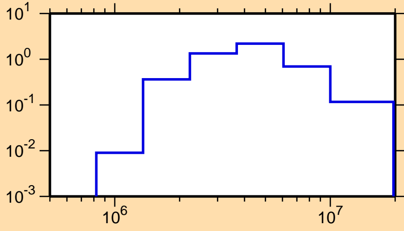
\sigma vs. E for ^{214}\text{Pb}(n,n\text{cont.})
