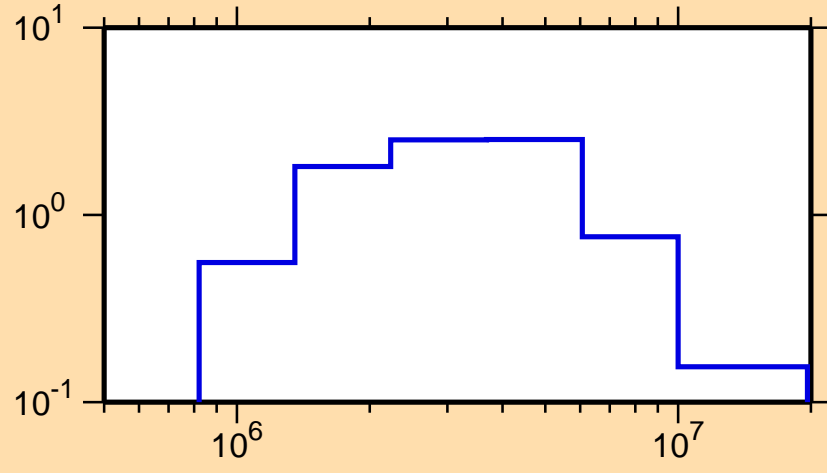
\sigma vs. E for ^{214}\text{Pb}(n,\text{inel.})
