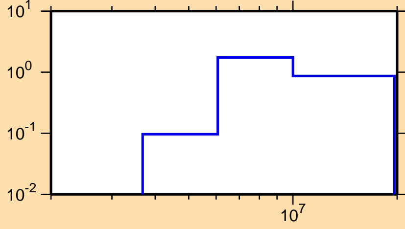
\sigma vs. E for ^{214}\text{Pb}(n,2n)
