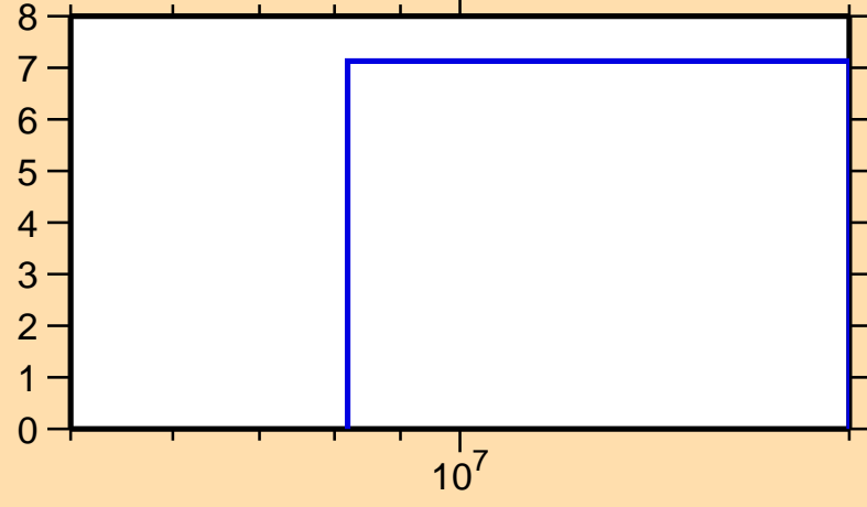
\Delta\sigma/\sigma vs. E for ^{214}\text{Pb}(n,\text{el.})
