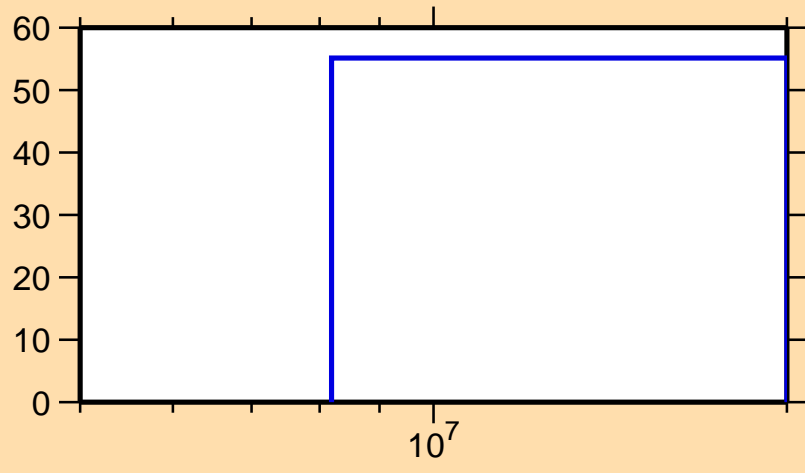
\Delta\sigma/\sigma vs. E for ^{214}\text{Pb}(n,n\text{cont.})
