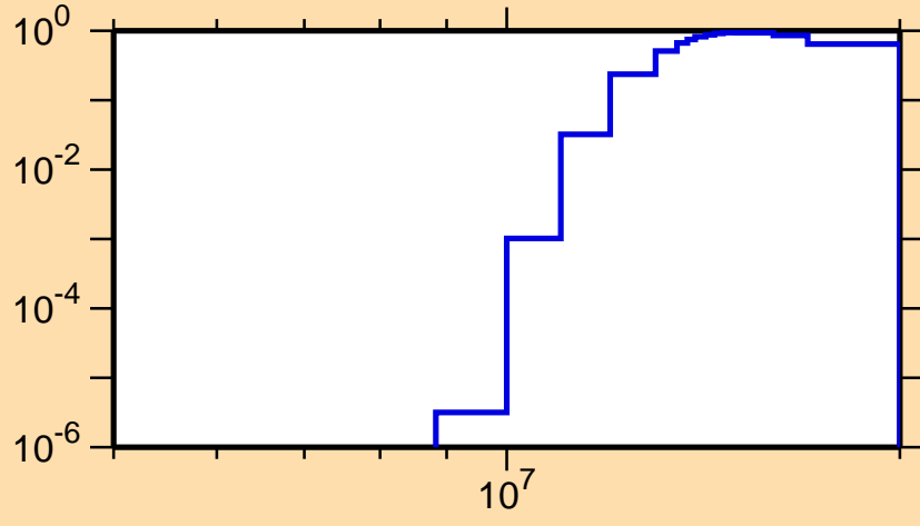
\sigma vs. E for ^{216}\text{Pb}(n,t)
