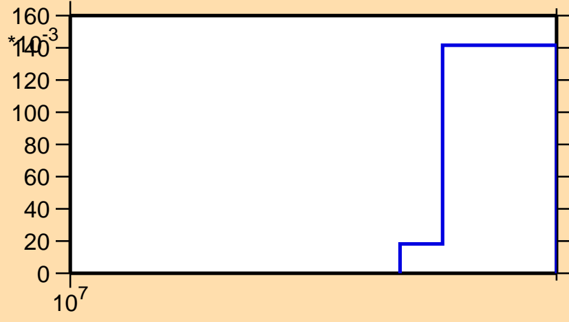
\sigma vs. E for ^{216}\text{Pb}(n,\text{nd})
