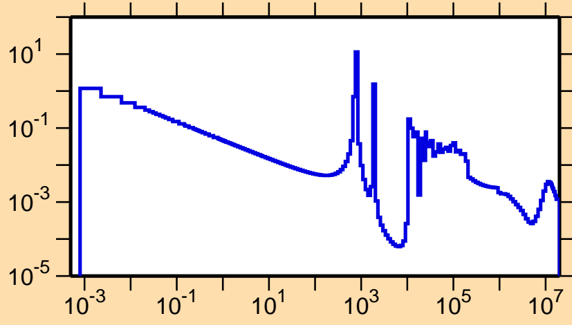
\sigma vs. E for ^{216}\text{Pb}(n,\gamma)
