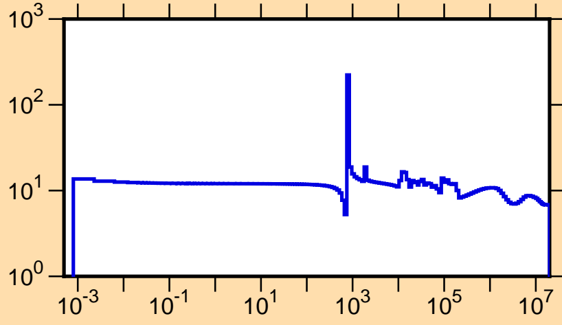
\sigma vs. E for ^{216}\text{Pb}(n,\text{tot.})
