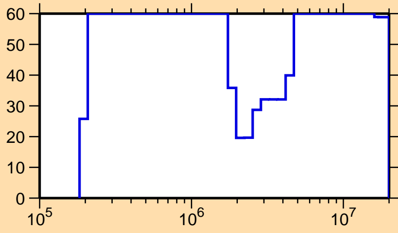
\Delta\sigma/\sigma vs. E for ^{216}\text{Pb}(n,\text{el.})
