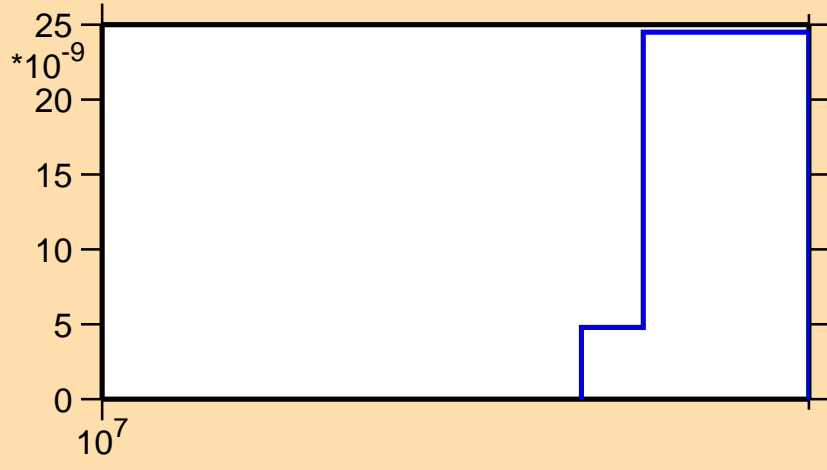
\sigma vs. E for ^{216}\text{Pb}(n,3n\alpha)
