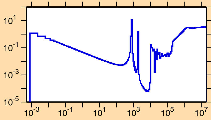
\sigma vs. E for ^{216}\text{Pb}(n,\text{nonel.})
