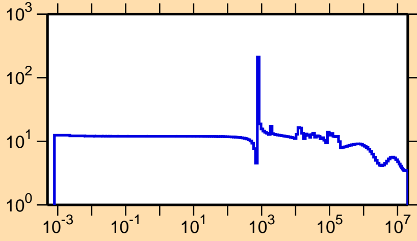
\sigma vs. E for ^{216}\text{Pb}(n,\text{el.})
