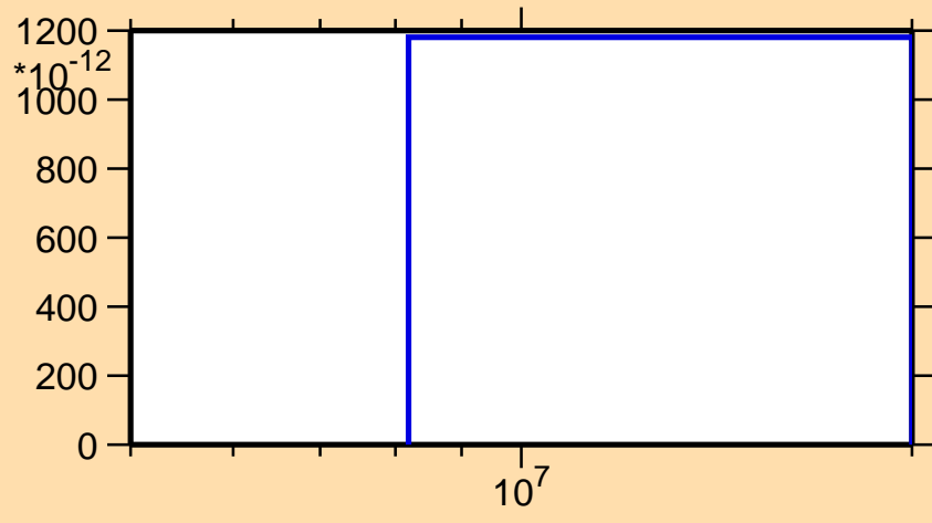
\sigma vs. E for ^{216}\text{Pb}(\text{mt } 11)
