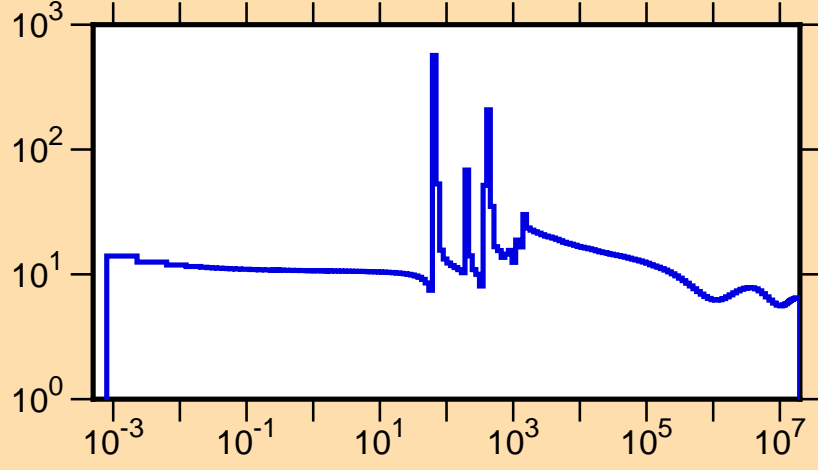
\sigma vs. E for ^{217}\text{Pb}(n,\text{tot.})
